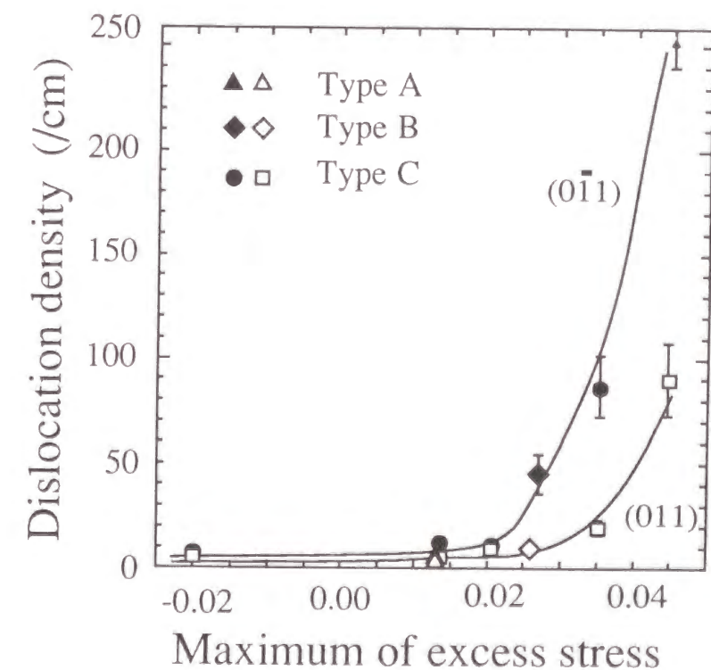
Figure 2-21 Dislocation density of (011)- and (0 \bar{1}1 )- direction as a function of maximum excess stress during growth.
