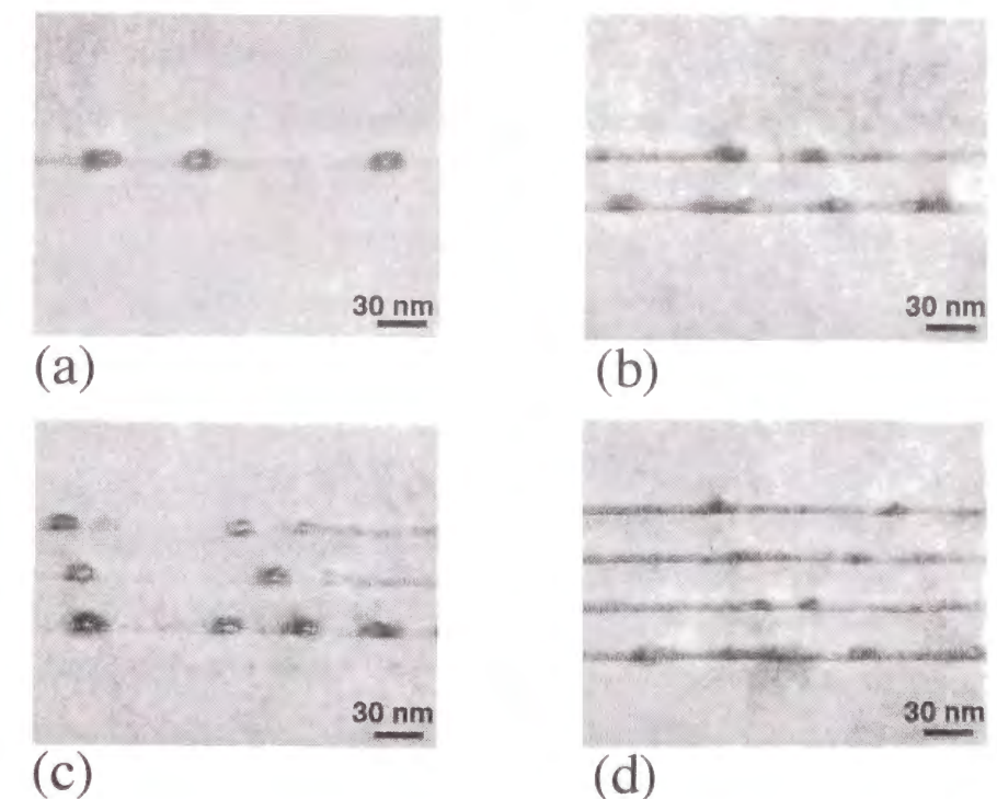
Figure 6-24 Cross-sectional transmission electron microscopy (TEM) image of InGaAs/GaAs quantum-dot layers: (a) single, (b) double, (c) triple, and (d) quadruple stacked structures. Dot layers were separated by 26-nm-thick GaAs barrier layers.
