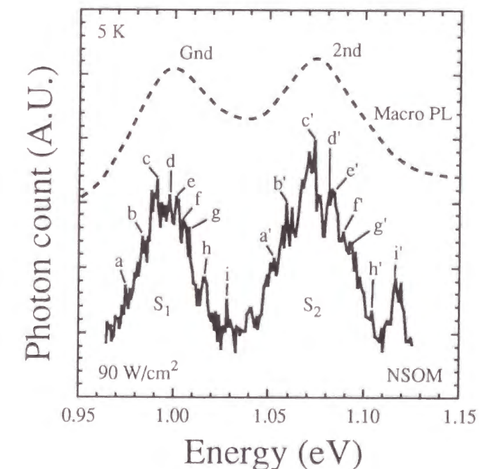
Figure 4-10 Photoluminescence spectra of the ALS dots by the near-field optical microscope. The excitation power was estimated to be 90\text{ W/cm}^2 . The spectra of macro-photoluminescence is shown by a dashed line. The two sets of multiple emission peaks in the NSOM spectra correspond to the ground-state ( S_1 ) and the first excited-state ( S_2 ) emission.
