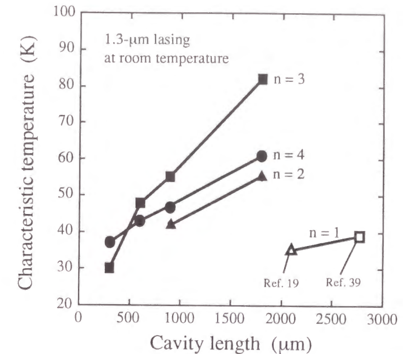
Figure 6-32 Characteristic temperature of 1.3- \mu\text{m} dot lasers at room temperature as a function of cavity length. Previous reported data where number of dot sheets was 1 are superimposed.
