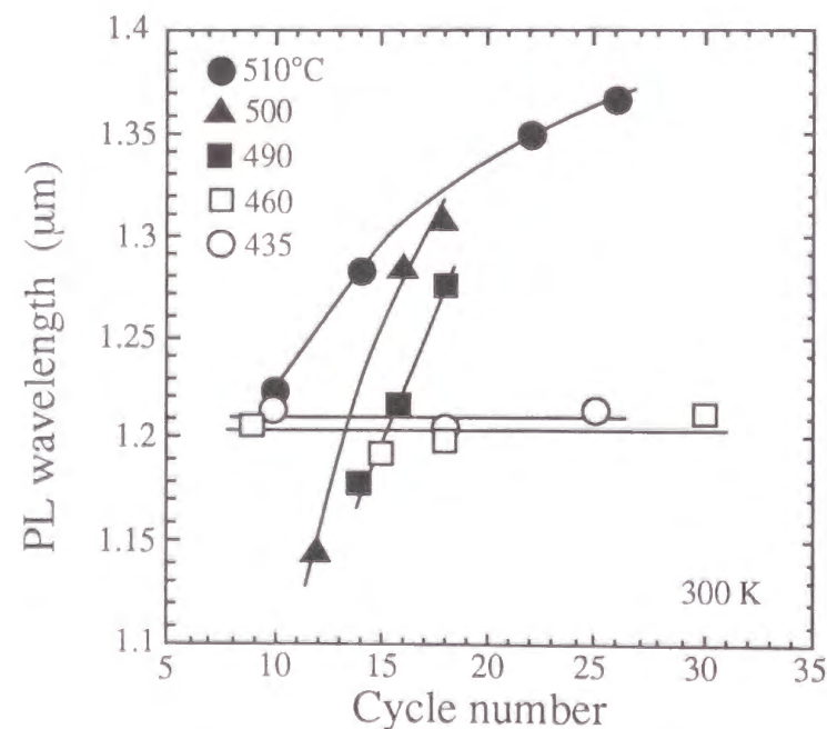
Figure 3-9 Peak wavelength of photoluminescence spectra as a function of the In - Ga- As cycle number grown at various temperatures. The relationship between the cycle number and the emission wavelength varies considerably between the two temperature ranges.
