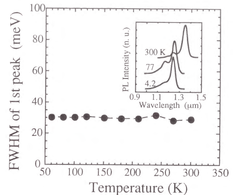
Figure 4-4 Photoluminescence spectrum width (FWHM) of the ALS dots as a function of temperature. The dots were grown using 12 cycles of the In-As-Ga-As alternate supply on an \text{In}_{0.05}\text{Ga}_{0.95}\text{As} buffer and capped with an \text{In}_{0.05}\text{Ga}_{0.95}\text{As} layer. Photoluminescence spectra at 4.2, 77 and 300 K are shown. The width of 30 meV is independent of temperature.
