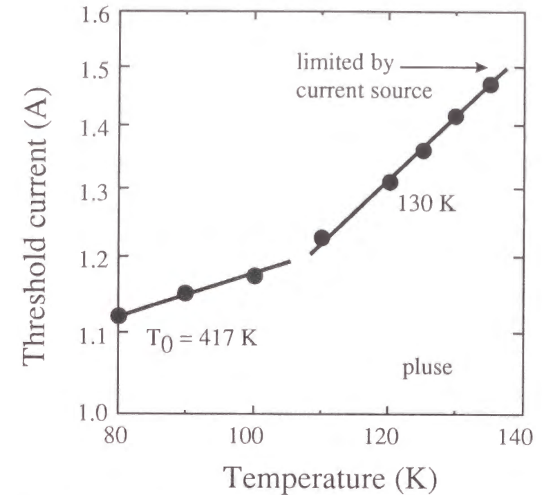
Figure 6-3 Threshold current of ALS-dot lasers as a function of temperature. Observation of lasing was limited by current source capacity. Over 400 K of characteristic temperature was obtained for the measurements below 100 K.
