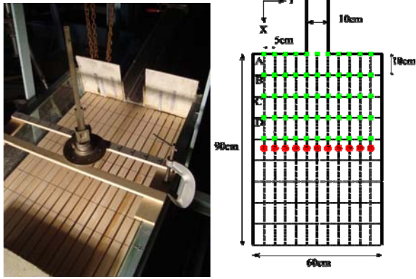
Fig.3 Observation points on the debris-flow breaker
