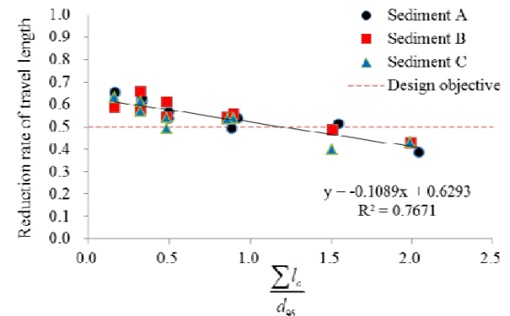
II. Relationship between reduction rate and \frac{\sum l_o}{d_{95}}
