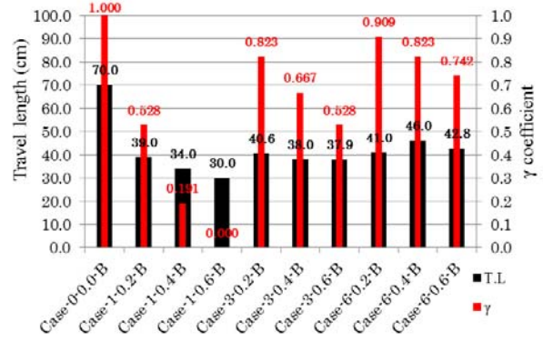
Fig.5 Compare to travel length and \gamma coefficient
