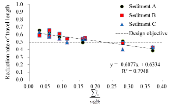
I. Relationship between reduction rate and \frac{\sum l_o}{width}
