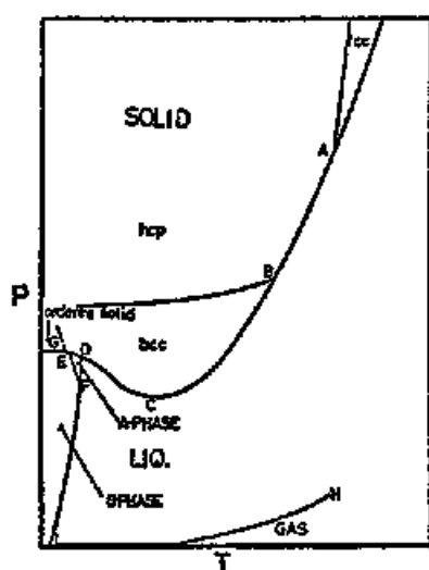
Fig.1 Phase Diagram of ^3\text{He}
