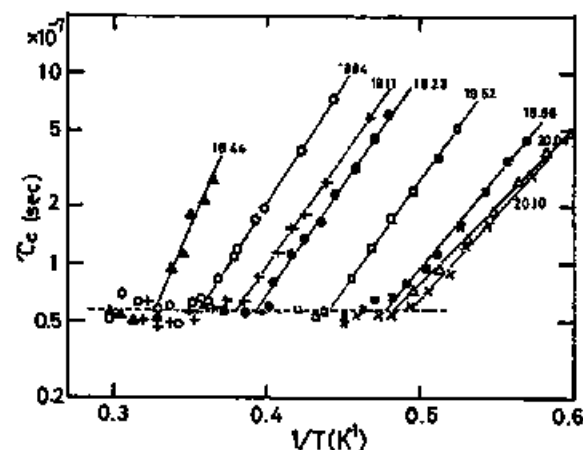
Fig. 1. Temperature dependence of the correlation time ( \tau_c ) of the motion of a ^3\text{He} spin in a 4.8% ^3\text{He} - ^4\text{He} mixture, obtained from the analysis of ^3\text{He} NMR relaxation data. The solid lines are the results of the least square fitting for the data in the solid phase. The dotted line is that for the data along the liquid-solid coexistence curve, in which the molar volume of the solid is continuously changing. The values of the molar volumes for the solid phase are included in the figure.
