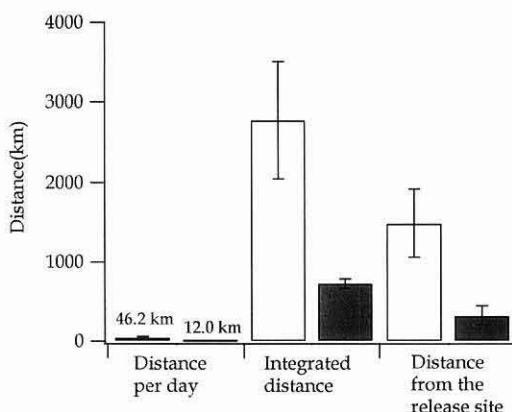
Fig. 4 Transport distance per day, integrated distance, and distance from the release site for loggerhead (open column) and green turtles (solid column) after 60 days.
