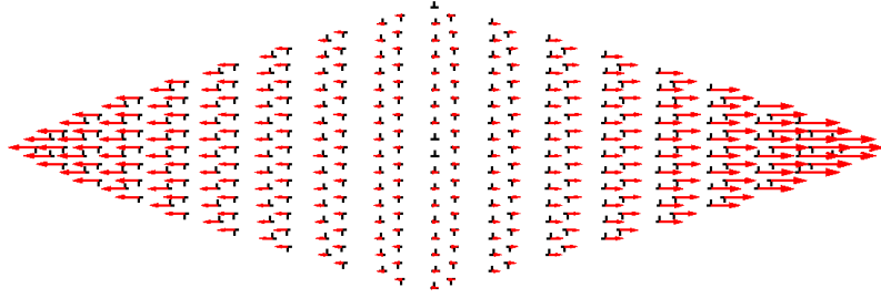
Fig. 6 Instability mode vector of the vein with N_v = 9 .
