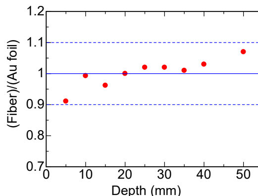
Fig. 3. Comparison between the thermal neutron flux measured by gold foil activation method and the optical fiber type neutron detector.
