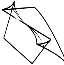
Scherbak surface (1, 3, 5)
