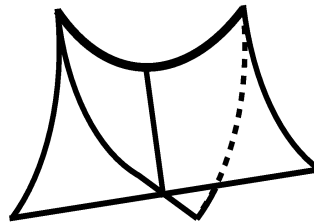
folded umbrella
