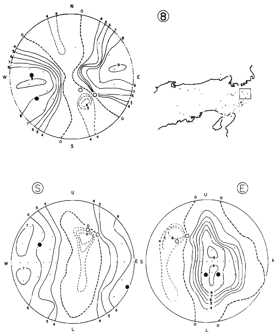
Fig. 15 (a) Smoothed radiation pattern of Region 8. The expression is the same as Fig. 7(a).
