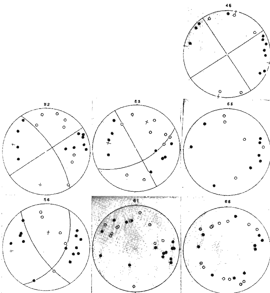
Fig. 10 (b) Individual fault plane solution and distribution of initial P motions projected by Wulff's net. The expression is the same as Fig.7(b) (Region 4)
