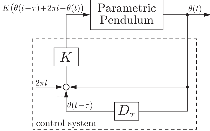
Figure 5.3: Block diagram of the proposed control for the periodic rotation inherent in the parametric pendulum (5.1).
