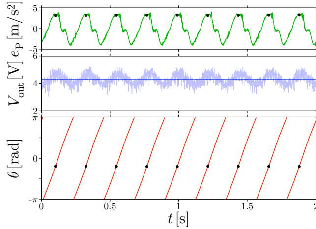
Figure 6.18: Energy scavenging by a periodic rotation of the mechanical pendulum with the DC motor from the vertical vibration. The vertical excitation is regulated to sinusoidal waveform with amplitude 3.4 \text{ m/s}^2 and frequency 4.5 \text{ Hz} . The electric load is resistance 500 \Omega .
