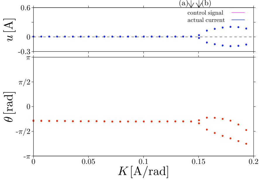
Figure 6.11: Bifurcation diagram with respect to the control gain K for the periodic rotation of the vertically excited mechanical pendulum under the start control. The vertical excitation is regulated to sinusoidal waveform with amplitude 1.1 \text{ m/s}^2 and frequency 2 \text{ Hz} . As for the control parameters, the delay time is fixed at the excitation period and the rotation number is unit. The data are measured through the stroboscopic observation.
