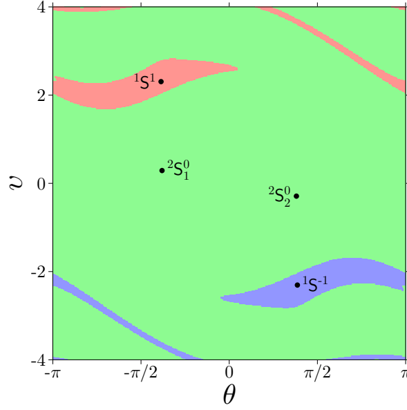
Figure 5.2: Domain of attraction for the parametric pendulum (5.1) at c = 0.1 , p = 0.5 , and \omega = 2 . The fixed points {}^1\mathbf{S}^{\pm 1} correspond to stable periodic rotations (1, \pm 1) , respectively. The pair of periodic points {}^2\mathbf{S}_{1,2}^0 denote a stable 2T_P -periodic libration.
