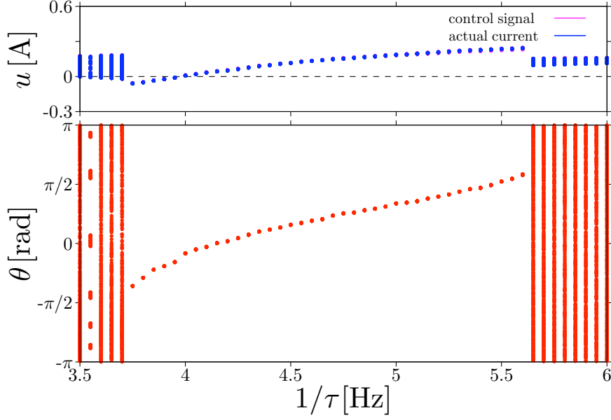
Figure 6.16: Bifurcation diagram of rotation with respect to the control frequency 1/\tau in the vertically excited mechanical pendulum under the start control. The vertical excitation is regulated to sinusoidal waveform with amplitude 2.2 \text{ m/s}^2 and frequency 4 \text{ Hz} . The control gain K is fixed at 0.14 \text{ A/rad} and the rotation number at unit. This diagram is measured by downward and upward shift of the control frequency from the excitation frequency 4 \text{ Hz} .
