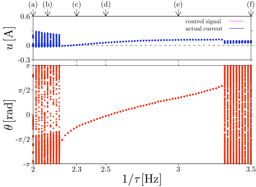
Figure 6.13: Bifurcation diagram of rotation with respect to the control frequency as the reciprocal of the delay time \tau in the vertically excited mechanical pendulum under the start control. The vertical excitation is regulated to sinusoidal waveform with amplitude 1.2 \text{ m/s}^2 and frequency 2.3 \text{ Hz} . The control gain is regulated to 0.072 \text{ A/rad} and the rotation number is fixed at unit. This diagram is measured by downward and upward shift of the control frequency from the excitation frequency 2.3 \text{ Hz} .
