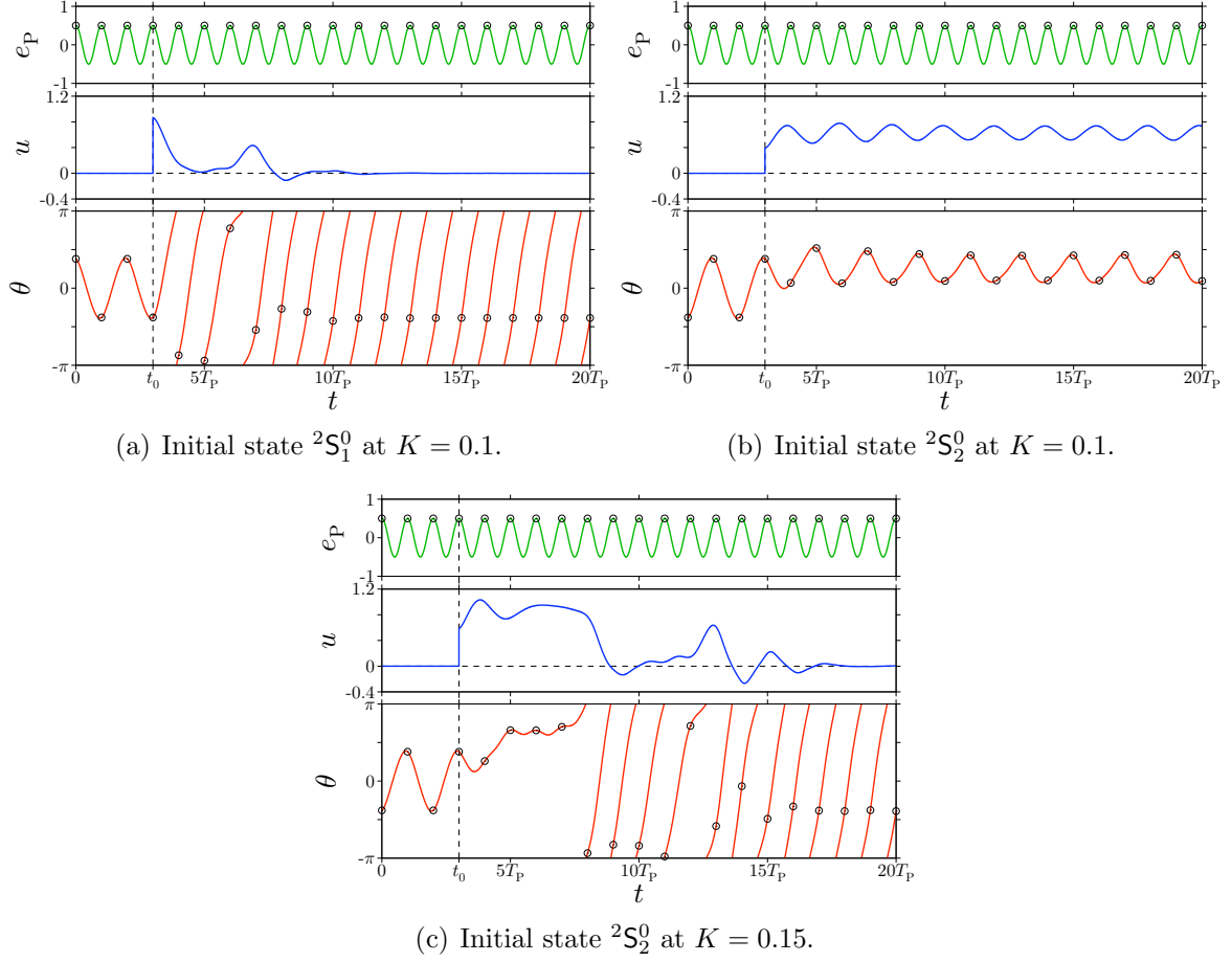
Figure 5.4: Behaviors of the controlled parametric pendulum (5.4). The other parameters are fixed at c = 0.1 , p = 0.5 , \omega = 2 , \tau = T_P = 2\pi/\omega , and l = 1 . The initial condition for the time delay component is set at the coexisting 2T_P -periodic libration. The start control is applied from t = t_0 = 3T_P = 3 \cdot 2\pi/\omega . The initial state is one of the periodic points corresponding to the 2T_P -periodic libration, namely {}^2S_{1,2}^0 shown in Fig. 5.2. The circles \odot on the curves denote the stroboscopic points at the excitation period T_P .
