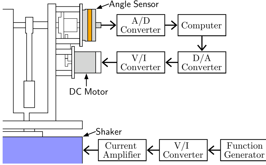
Figure 6.4: Schematic diagram of the experimental setup.
