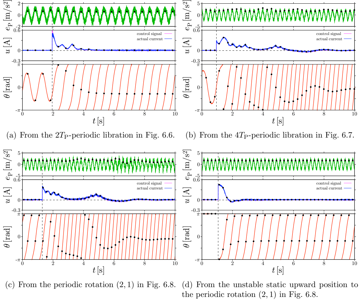
Figure 6.10: Start control of the vertically excited mechanical pendulum assembled at Setting 2 in Table 6.1. The vertical excitation is regulated as the same as Figs. 6.6, 6.7, and 6.8. As the control parameters, the control gain K is 0.072 A/rad and the delayed time \tau is the same as the excitation period in (a) and (b). In (c), the control gain K is increased to 0.11 A/rad. In (d), the delay time \tau is regulated to twice the period in order to target the periodic rotation (2, 1). The rotation number is fixed at l = 1 .
