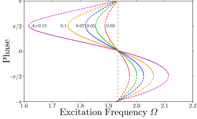
(a) Phase.
