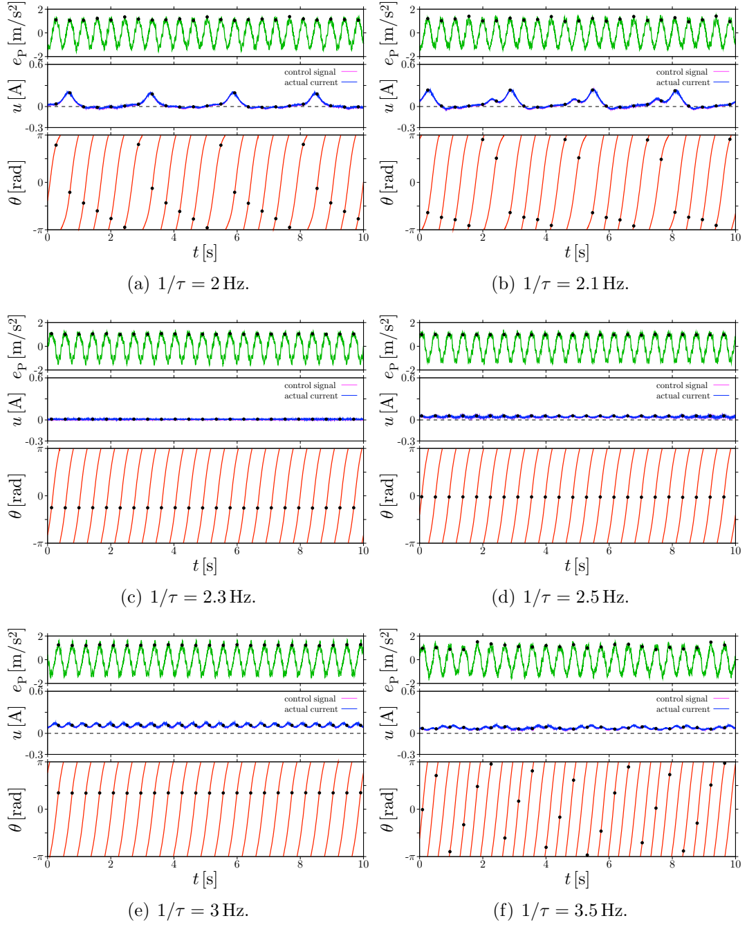
Figure 6.14: Behaviors of the vertically excited mechanical pendulum under the start control at different delay time in Fig. 6.13.
