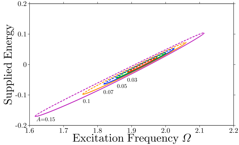
Figure 4.2: Response curves for the energy supplied by the periodic excitation in the system (4.1) at k = 0.1 and N = 0.2 . The supplied energy is calculated from the last term on the right-hand side of Eq. (4.9). The solid lines correspond to completely stable rotations and the dashed lines directly unstable ones [78]. The detailed classification of the stability of these periodic rotations is explained in the appendix of Chapter 3.
