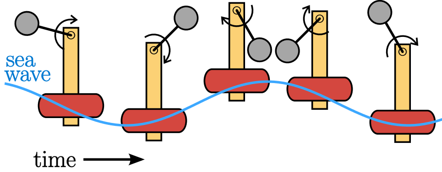
Figure 1.1: Conceptual diagram of energy extraction from the heave motion of sea wave by the parametric pendulum.
