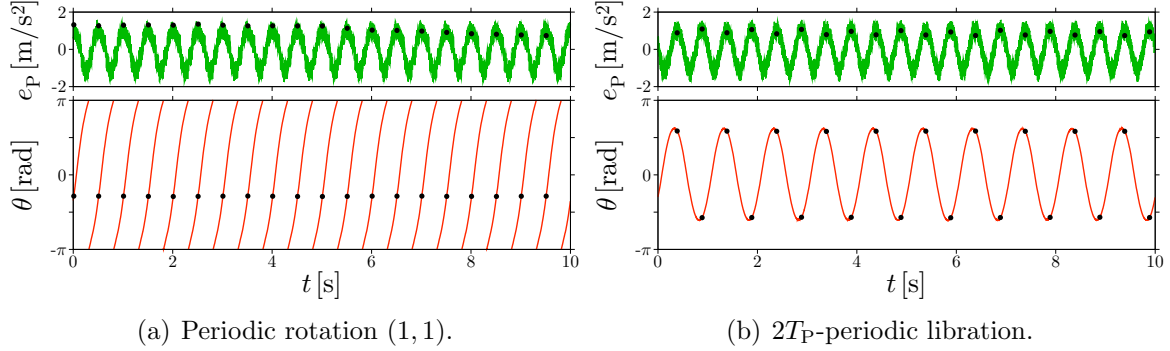
Figure 6.6: Steady motions of the mechanical pendulum at sinusoidal excitation with amplitude 1.1 \text{ m/s}^2 and frequency 2 \text{ Hz} . The mechanical pendulum is assembled with the largest moment of inertia.
