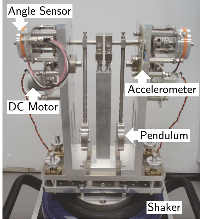
Figure 6.3: Photograph of the experimental setup for the parametric pendulum. The experimental setup consists of the mechanical rig supporting the pendulums mounted on the electromagnetic shaker which generates vertical excitation.
