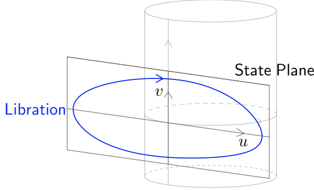
Figure 2.4: Librational limit cycle on the state plane of the van der Pol oscillator (2.16), where v = du/dt . Libration existing on the cylindrical state space can exist on the state plane.
