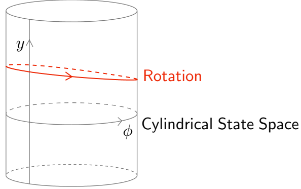
Figure 2.6: Rotational limit cycle in the cylindrical state space of the phase-locked system, where y = d\phi/dt .
