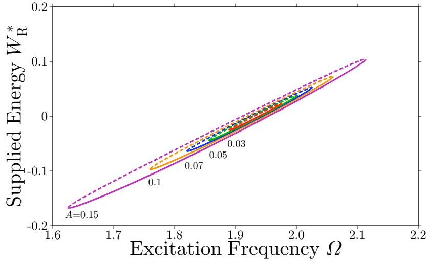
Figure 4.4: Response curves for the energy W_R^* supplied by the periodic excitation by using Eqs. (4.8) and W_R^* = -\pi a_R^* A \sin(\theta_R^* + \delta_R^*) at k = 0.1 and N = 0.2 . The solid lines correspond to stable equilibrium points and the dashed lines unstable ones.
