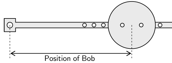
Figure 6.2: Schematic illustration of the mechanical pendulum. The pendulum is constructed by inserting the rod in the hole of the bob and fixing the position. The position of the bob is described as center-to-center distance between the rotary shaft and the bob.
