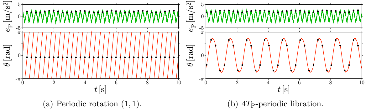
Figure 6.7: Steady motions of the mechanical pendulum at sinusoidal excitation with amplitude 2.1 \text{ m/s}^2 and frequency 3.5 \text{ Hz} . The mechanical pendulum is assembled with the largest moment of inertia.
