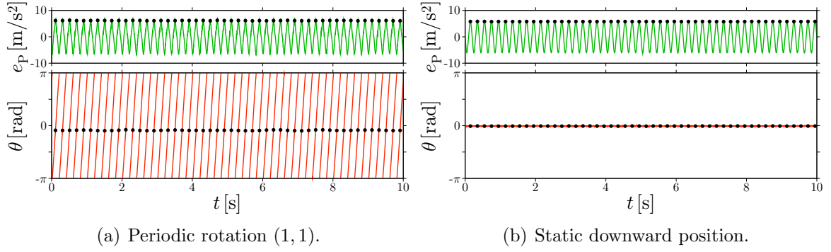
Figure 6.5: Steady states of the vertically excited mechanical pendulum with the smallest moment of inertia. The vertical excitation of the shaker is regulated to sinusoidal waveform with amplitude 5.6 \text{ m/s}^2 and frequency 5 \text{ Hz} . The dots denote the stroboscopic points at every excitation period.
