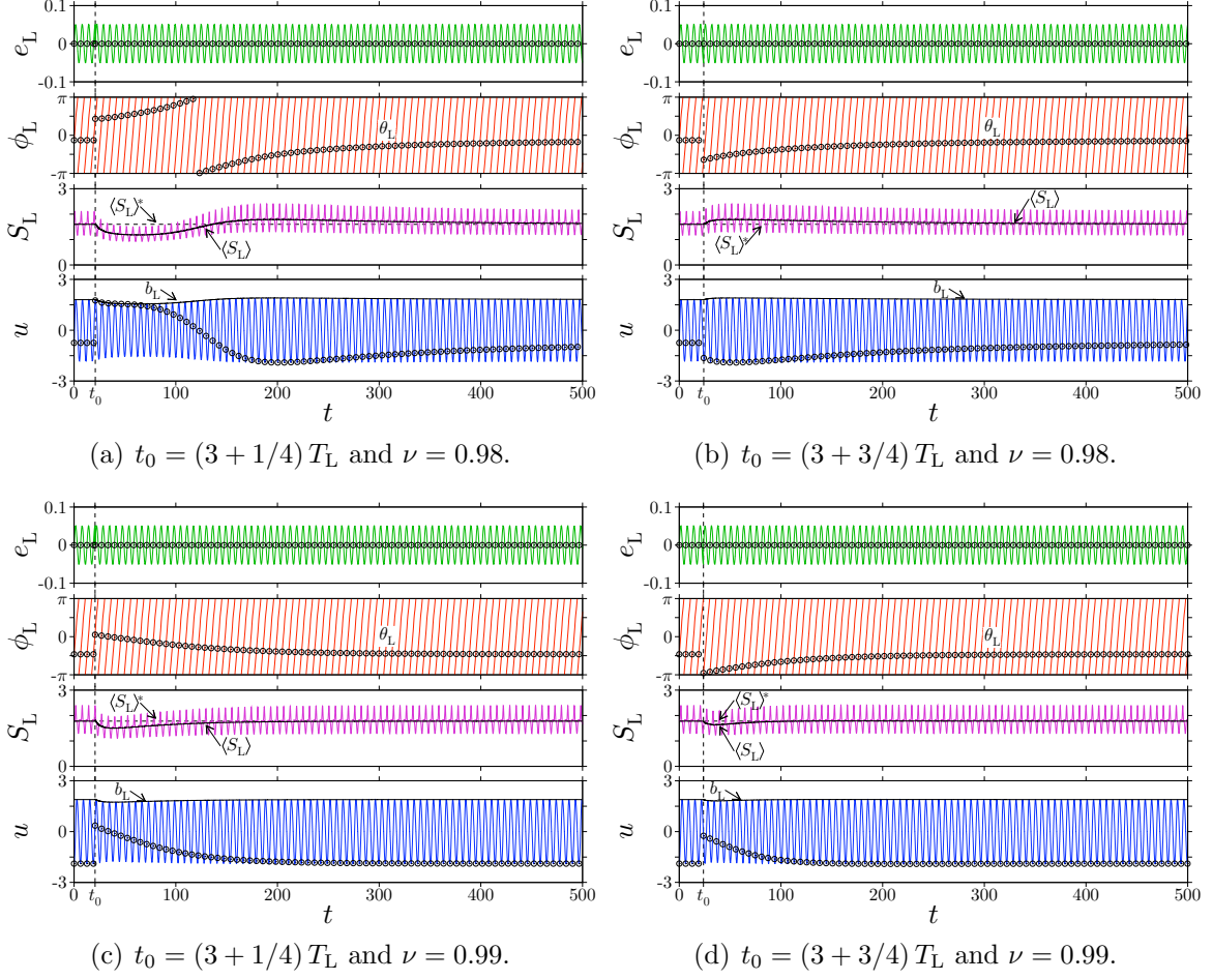
Figure 3.6: Stored energy and phase in the frequency entrainment of libration in the system (3.1) at \mu = 0.15 , \beta = \gamma = 4/3 , and B = 0.05 . The phase of the periodic excitation e_L is reset at t = t_0 , and then the transient regime of the frequency entrainment appears. The solid lines on the waveforms of u and S_L denote the amplitude and the time average of S_L , respectively. The dashed lines of S_L represent the time average at the entrained libration. Since these lines correspond to b_L , \langle S_L \rangle , and \langle S_L \rangle^* , we indicate these lines by using the corresponding notation. The phase \theta_L is estimated from the stroboscopic points \odot of \tan^{-1}(\nu u/v) =: \phi_L .
