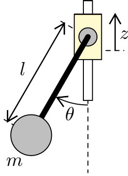
Figure 2.8: Model of a vertically excited pendulum.
