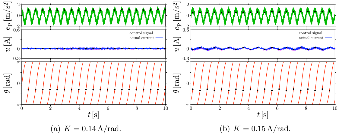
Figure 6.12: Behaviors of the vertically excited mechanical pendulum under the start control at the different control gain K in Fig. 6.11.
