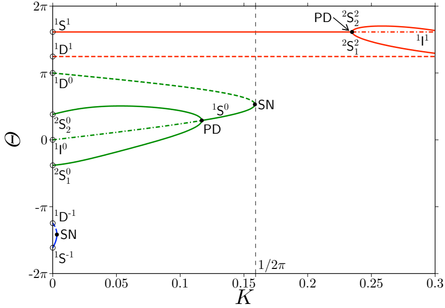
Figure 5.6: Bifurcation diagram with respect to the control gain K in the controlled parametric pendulum (5.4) at c = 0.1 , p = 0.5 , \omega = 2 , \tau = T_P = 2\pi/\omega , and l = 1 . PD denotes the period-doubling bifurcation and SN the saddle-node bifurcation. The type of line shows the stability of the periodic states; the solid lines denote completely stable states, the dashed lines directly unstable ones, and the chain lines inversely unstable ones. The detailed classification of the stability is explained in the appendix of Chapter 3.
