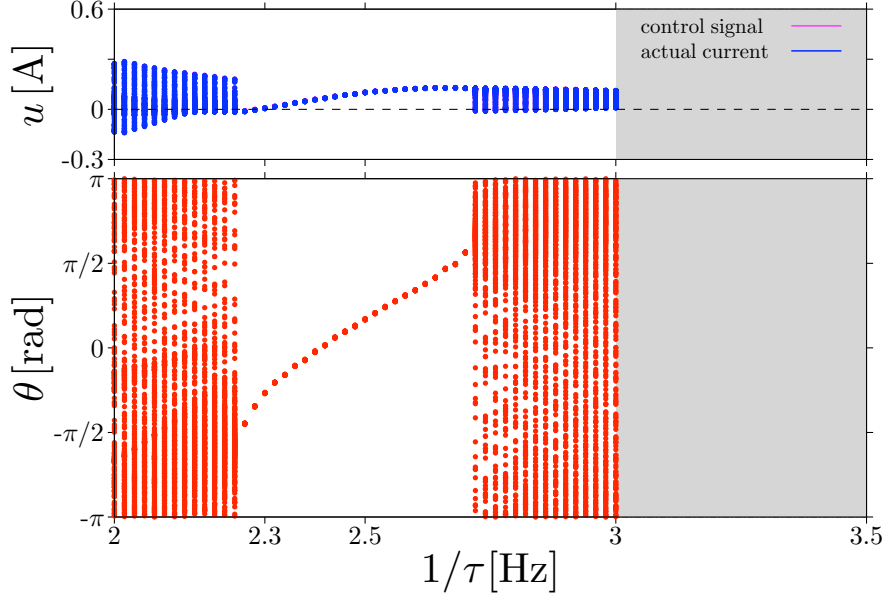
Figure 6.15: Bifurcation diagram of rotation with respect to the delay time \tau in the vertically excited mechanical pendulum with the start control. The vertical excitation is regulated to sinusoidal waveform with amplitude 1.2 \text{ m/s}^2 and frequency 2.3 \text{ Hz} . The control gain is 0.14 \text{ A/rad} and the rotation number at unit.
