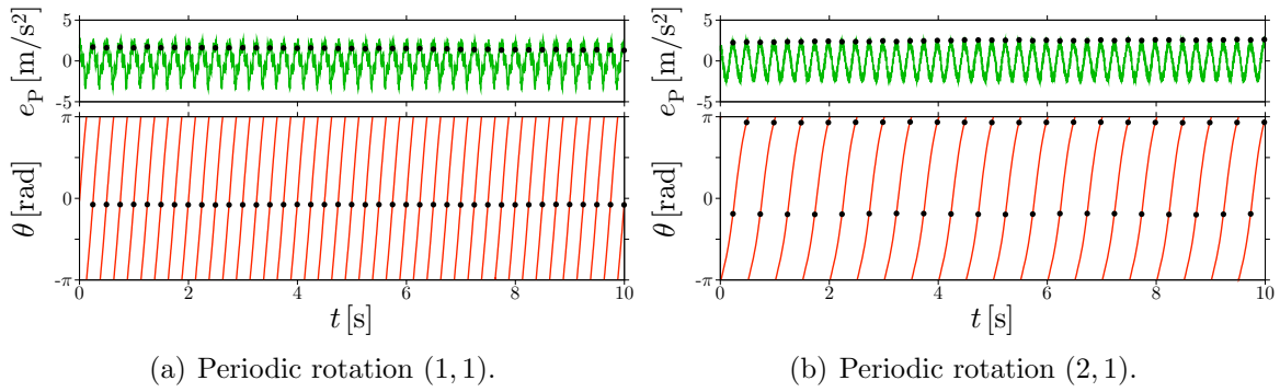
Figure 6.8: Two periodic rotations of the mechanical pendulum at sinusoidal excitation with amplitude 2.0 \text{ m/s}^2 and frequency 4 \text{ Hz} . The mechanical pendulum is assembled with the largest moment of inertia. The periodic rotations have rotation frequency different from each other.
