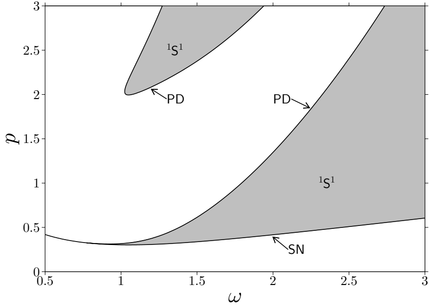
Figure 5.1: Existence domain of the periodic rotations (1, 1) in the excitation parameter space (p, \omega) for the parametric pendulum (5.1) at c = 0.1 . SN denotes the saddle-node bifurcation and PD the period-doubling bifurcation. The gray corresponds to the existence domain of the periodic rotations (1, 1) .
