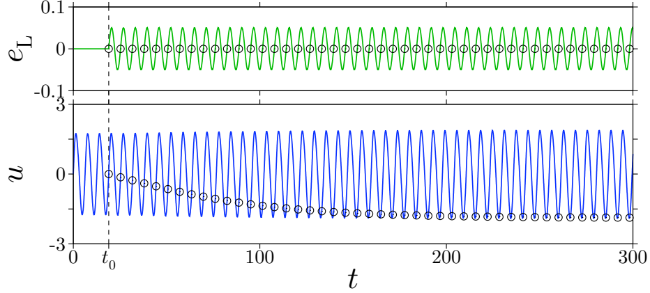
Figure 3.1: Frequency entrainment of libration in the system (3.1) at \mu = 0.15 , \beta = \gamma = 4/3 , B = 0.05 , and \nu = 0.99 . The periodic excitation e_L(t - t_0) = B \sin\{\nu(t - t_0)\} is applied from t = t_0 . The convergence of the stroboscopic points, denoted by the circles \odot , shows that the librational limit cycle is entrained by the periodic excitation.
