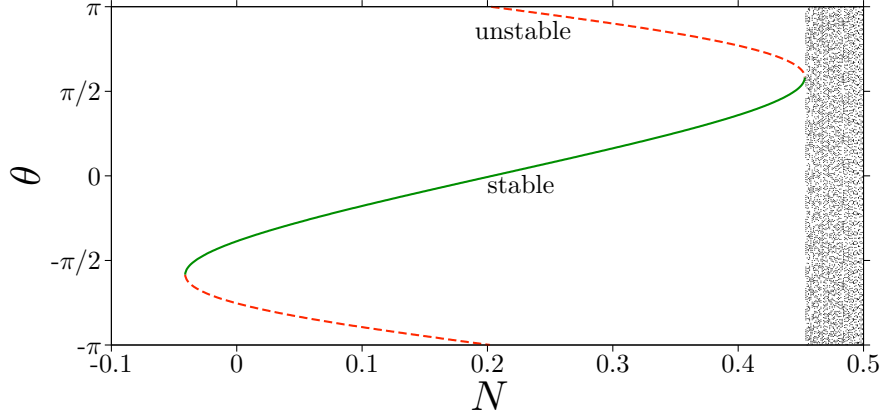
Figure 6.17: Bifurcation diagram of rotation with respect to the torque N in the driven parametric pendulum (6.1) at c = 0.1 , p = 0.5 , and \omega = 2 . The branches consist of the stroboscopic points.
