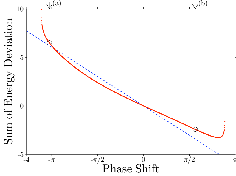
Figure 4.7: Relationship between the total of the deviation of the stored energy and the phase shift in the system (4.1) at k = 0.1 , N = 0.2 , A = 0.05 , and \Omega = 1.93 . The dashed line is the theoretical result obtained from Eq. (4.15), and the dots show the numerical one from Eq. (4.1). The arrows (a) and (b) show the situations in Figs. 4.6(a) and (b), respectively.
