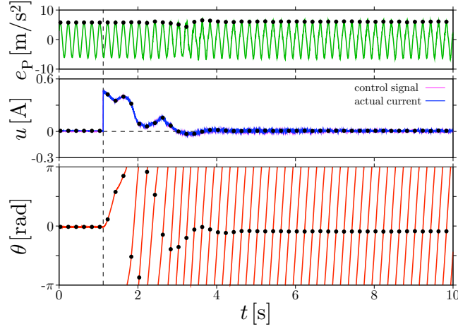
Figure 6.9: Start control of the vertically excited mechanical pendulum from the static downward position to the periodic rotation. The mechanical pendulum is assembled at Setting 1 in Table 6.1. In order to generate the inherent periodic rotation, the vertical excitation is regulated to sinusoidal waveform with amplitude 5.6 \text{ m/s}^2 and frequency 5 \text{ Hz} . As the control parameters, the control gain K is 0.072 \text{ A/rad} , the delayed time \tau is the same as the excitation period 1/(5 \text{ Hz}) = 2 \text{ s} , and the rotation number is fixed at l = 1 . The vertical dashed line indicates the beginning time of the start control.
