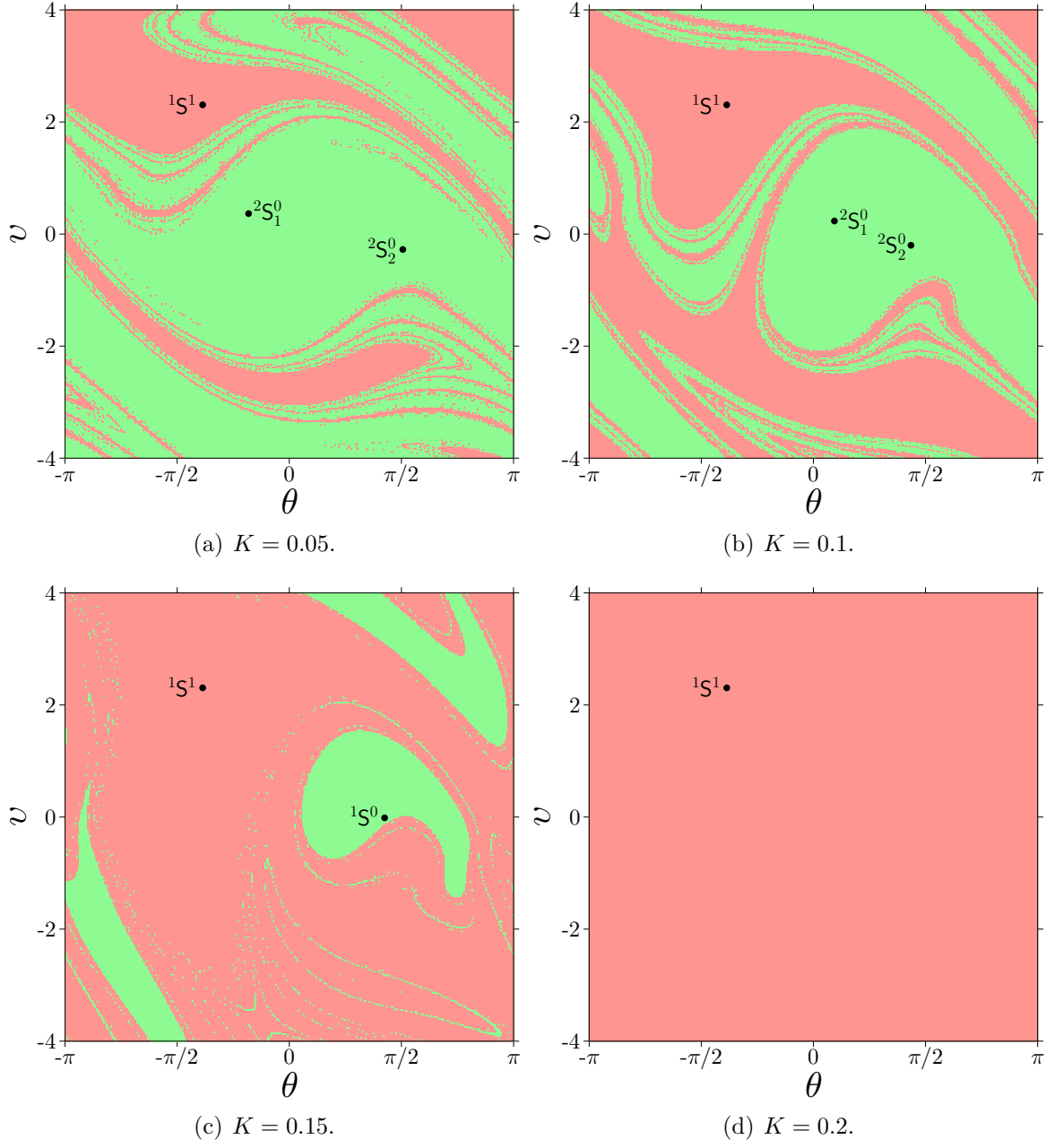
Figure 5.5: Domain of attraction for the controlled parametric pendulum (5.4) at c = 0.1 , p = 0.5 , \omega = 2 , \tau = T_P = 2\pi/\omega , and l = 1 . The start control is applied from t = 0 . The initial condition for the time delay component is given as the inherent behavior of the parametric pendulum (5.1) for t < 0 . The target rotation is indicated by the fixed point ^1S^1 .
