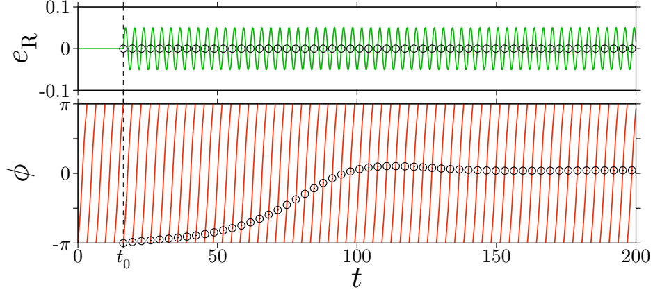
Figure 4.1: Frequency entrainment of rotation in the system (4.1) at k = 0.1 , N = 0.2 , A = 0.05 , and \Omega = 1.93 . The periodic excitation e_R(t - t_0) = A \sin\{\Omega(t - t_0)\} is applied from t = t_0 . The convergence of the stroboscopic points, denoted by the circles \odot , shows that the rotational limit cycle is entrained by the periodic excitation.
