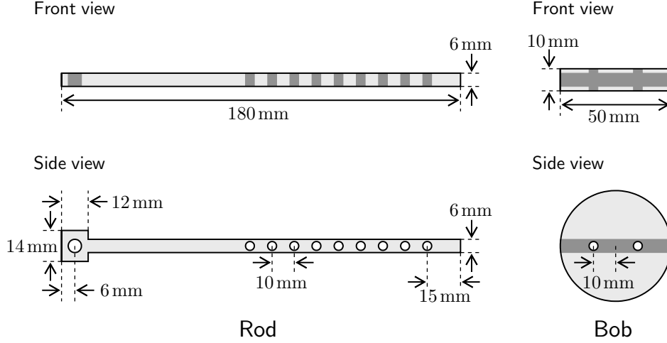
Figure 6.1: Schematic illustration of the parts of the mechanical pendulum: the rod and the bob. The gray corresponds to the holes.
