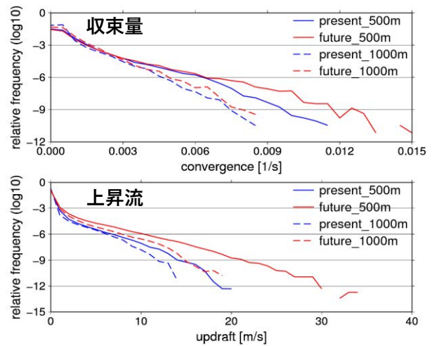
Fig. 11. The relative frequency of convergence (upper) and updraft (lower).
