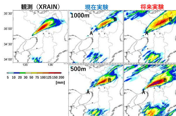
Fig. 4. Six-hour total rainfall of observation (left), present (middle) and future (right) experiments. Upper (lower) shows 1000m (500m) resolution results.
