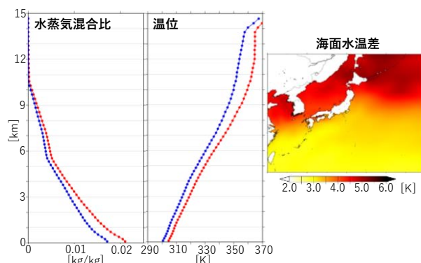
Fig. 3. Global warming increment. Vertical profile of water vapor mixing ratio (left) and potential temperature (middle) averaged over the area of 135°E ~ 136.5°E and 34.5°N ~ 35.5°N at initial time (red/ blue: future/ present), and spatial distribution of future change for sea surface temperature (right).
