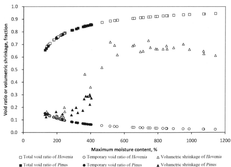
Figure 1. Changes of void ratio and volumetric shrinkage of archaeological waterlogged wood.
