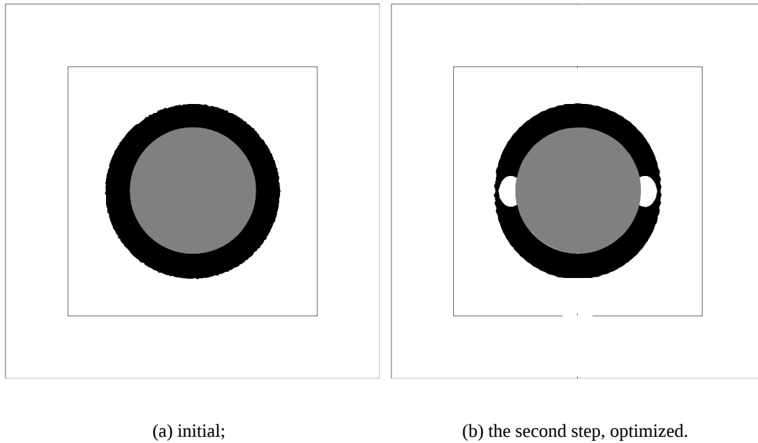
Figure 5-14: Configurations of the optimization in effective mass density minimization problem targeting 1300 Hz.
