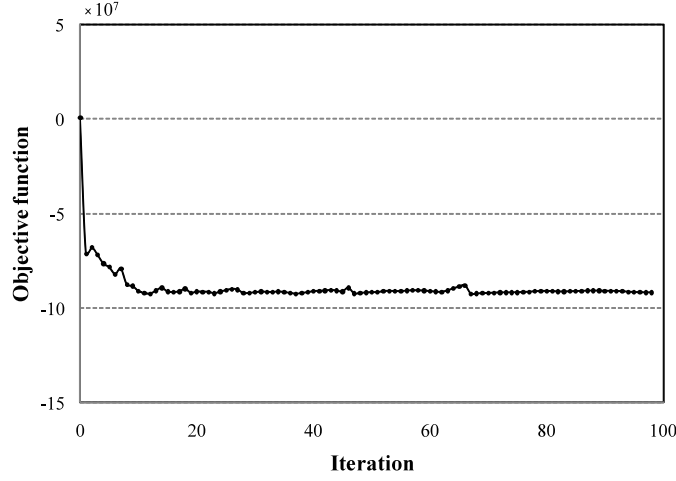
Figure 4-10: Convergence history of objection function of the second step optimization for effective bulk modulus minimization problem based on ring initial shape targeting 1550 Hz.
