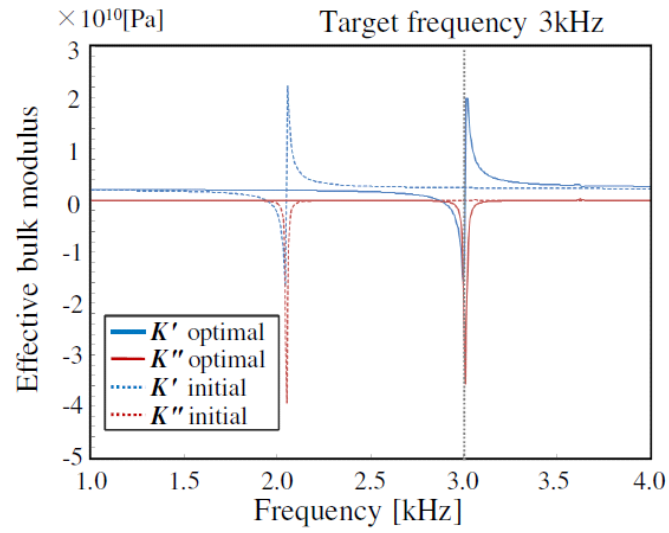
Figure 4-19: Effective bulk modulus curves for effective bulk modulus minimization problem targeting 3000 Hz.
