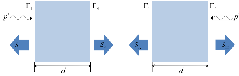
Figure 5-4: The illustrations of S-parameters.
