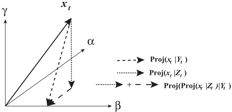
Figure 2.4: The relationships between Z_t and Y_T . \alpha \oplus \beta \oplus \gamma : the entire probability space and \alpha \oplus \beta : the probability space of Z_t , \beta : the probability space of Y_t
