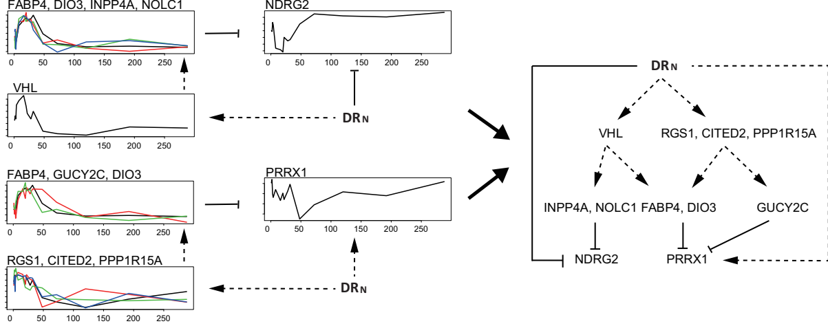
Figure 7.12: An example for integrating obtained pathways. Two pathways in the left are integrated to the gene network in the right. Arrows in this figure are the same as those in Fig. 7.6.
