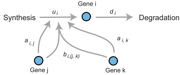
Figure 4.1: An example of the combinatorial transcription model regarding the i th gene. A gene undergoes synthesis and degradation processes, and its synthesis process is regulated through individual effects a_{i,j} , a_{i,k} and a combinatorial effect b_{i,(j,k)} .
