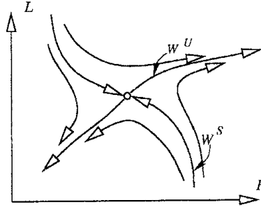
Fig. 4. The phase portrait
