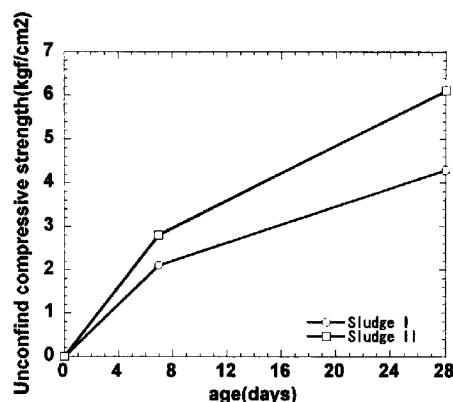
Fig. 3 Unconfined strength of treated sludge
