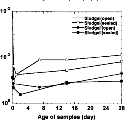
Fig. 4 pH changes of samples during curing
