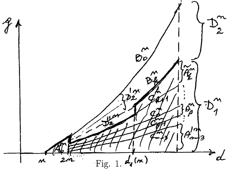
The hashurated domain in D_1^n (a non-lacunary domain).
