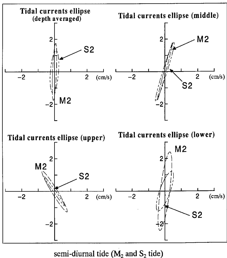
Fig.5 Tidal currents ellipses (diurnal and semi-diurnal tides)
