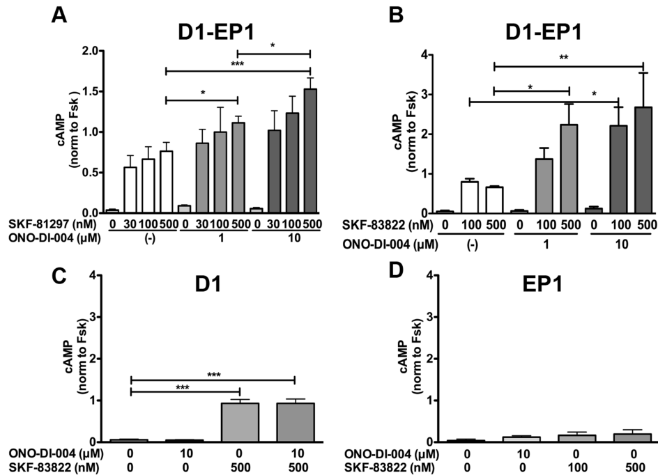
Figure 3.1. (Ehrlich et al., 2013). In HEK-293T cells, EP1 receptor activation enhances D1 receptor induced cAMP production. (A, B) EP1 receptor activation mediated enhancement of D1 receptor-induced cAMP response. HEK-293T cells overexpressing D1 and EP1 receptors (“D1-EP1”) were treated for 5 minutes with either a D1 agonist (SKF-81297 in (A) and SKF-83822 in (B)) in the presence or absence of an EP1 agonist (ONO-DI-004) as indicated. Intracellular cAMP levels were determined using a cAMP enzyme immunoassay and normalized to the cAMP level induced by 10 μM forskolin (Fsk). n = 5-6 for each column in (A) and n = 4-5 for each column in (B). (C) In D1 receptor alone expressing cells ONO-DI-004 lacks an effect on D1-induced cAMP response. As indicated, either SKF-83822, ONO-DI-004 or both agonists were added to the HEK-293T cells overexpressing D1 receptors alone (“D1”). cAMP levels were determined as described above. n = 6 for each column. (D) Cells which do not overexpress D1 receptors lack an effect of SKF-83822 and ONO-DI-004 on the cAMP level. As indicated, SKF-83822, ONO-DI-004, or both agonist treatments were applied to HEK-293T cells overexpressing EP1 receptors alone (“EP1”). cAMP levels were determined as above. n = 3 for each column. * P < 0.05 , ** P < 0.01 , *** P < 0.001 for Newman-Keuls multiple comparison tests following one-way analysis of variance.
