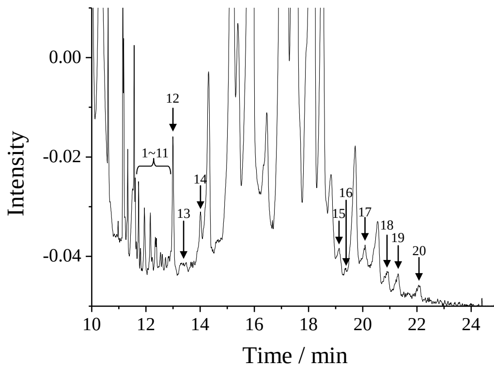
1 Figure 6. Detection of minor glycans obtained from AGP by LVSEP-CZE. 20 peaks 2 indicated with arrows could not be detected in conventional CZE. 3
