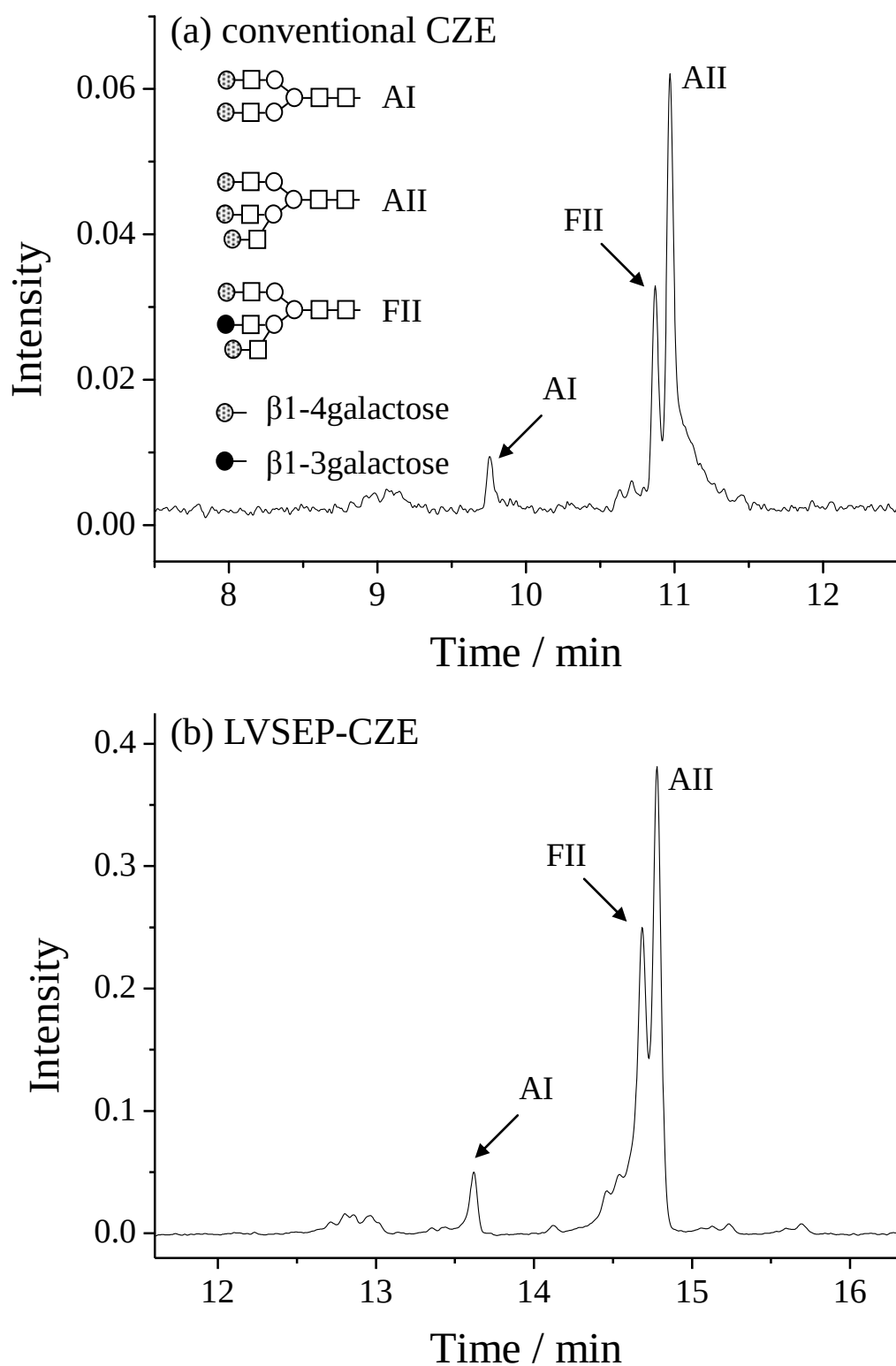
1 Figure 4. Electropherograms of fetuin glycans obtained in (a) conventional CZE and (b) 2 LVSEP-CZE. Sample concentration in LVSEP-CZE was 100-fold lower than that in 3 conventional CZE.
