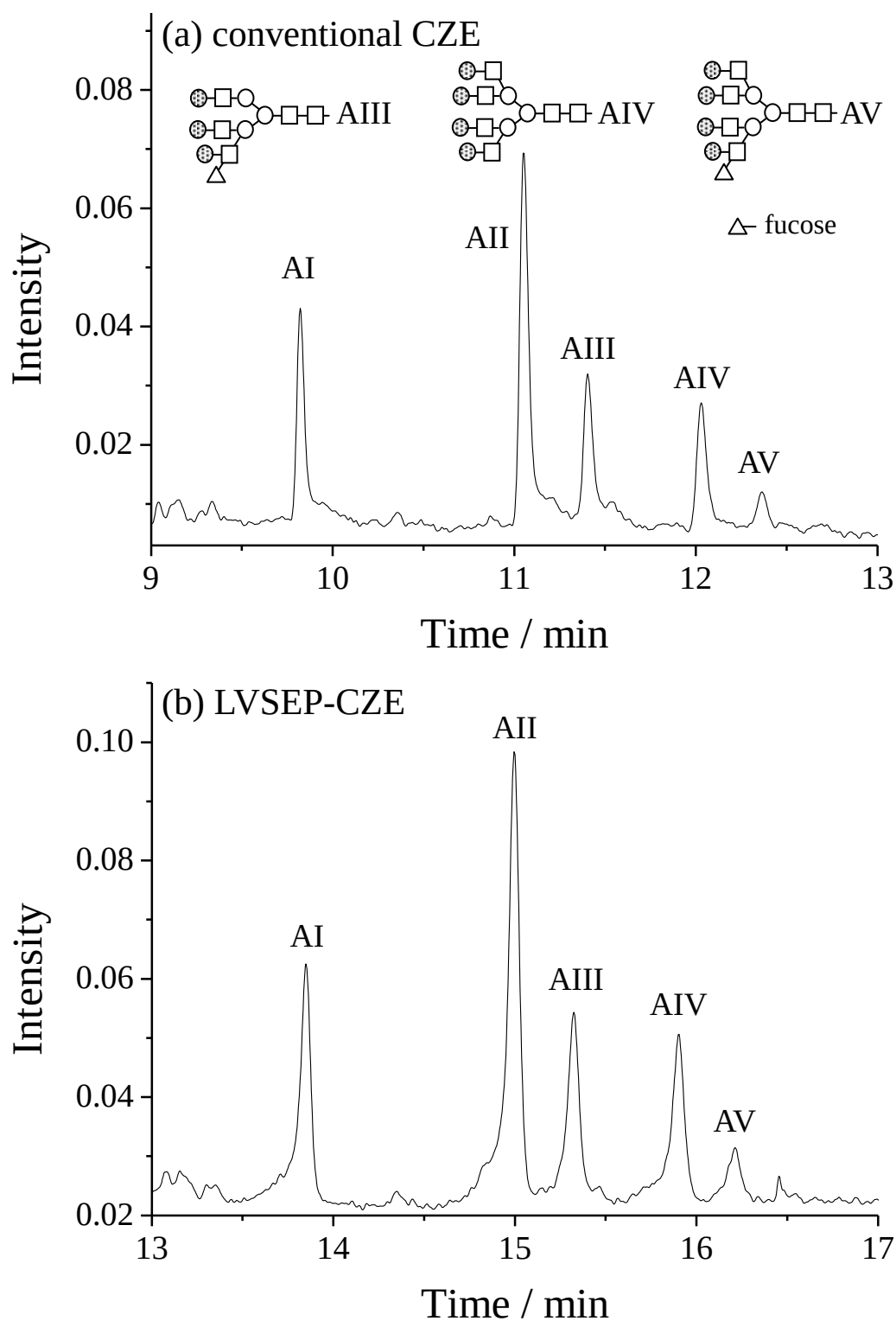
1 Figure 5. (a) Conventional CZE and (b) LVSEP-CZE analyses of glycans obtained 2 from AGP. Sample concentration in LVSEP-CZE was 400-fold lower than that in 3 conventional CZE.
