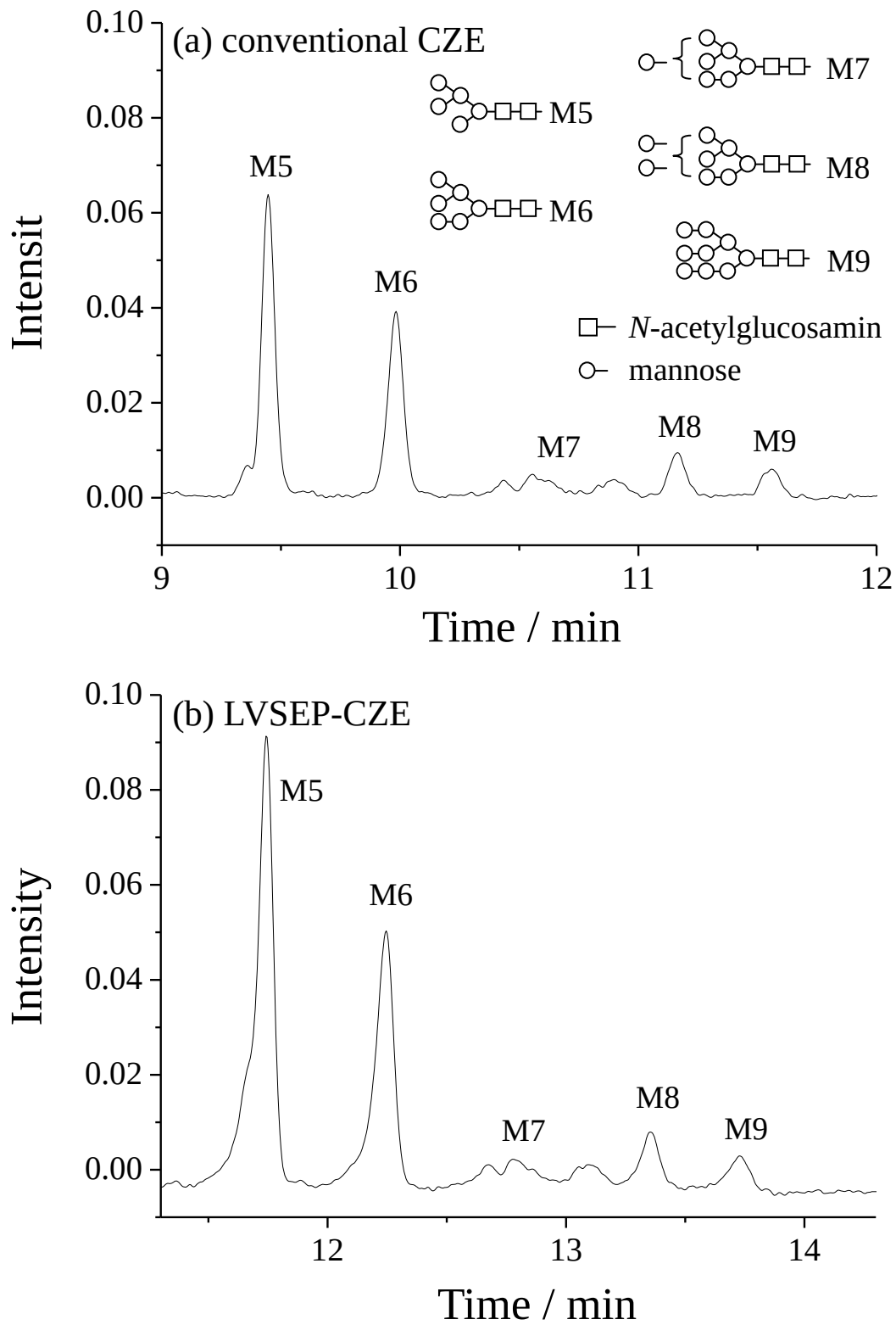
Figure 3. (a) Conventional CZE and (b) LVSEP-CZE analyses of oligosaccharides released from ribonuclease B. Sample concentration in LVSEP-CZE was 500-fold lower than that in normal CZE.
