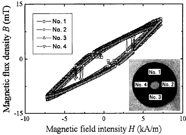
Fig. 2. Photograph and magnetic hysteresis curves (77.3K) of BSCCO-2223 bulk disk. Hysteresis curves are measured on different four points (see the photograph).
