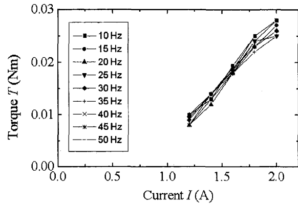
Fig. 5. Current versus torque characteristics of the HTS hysteresis motor.
