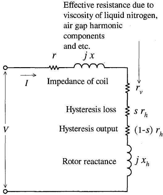
Fig. 3. Equivalent circuit of the HTS hysteresis motor per phase.
