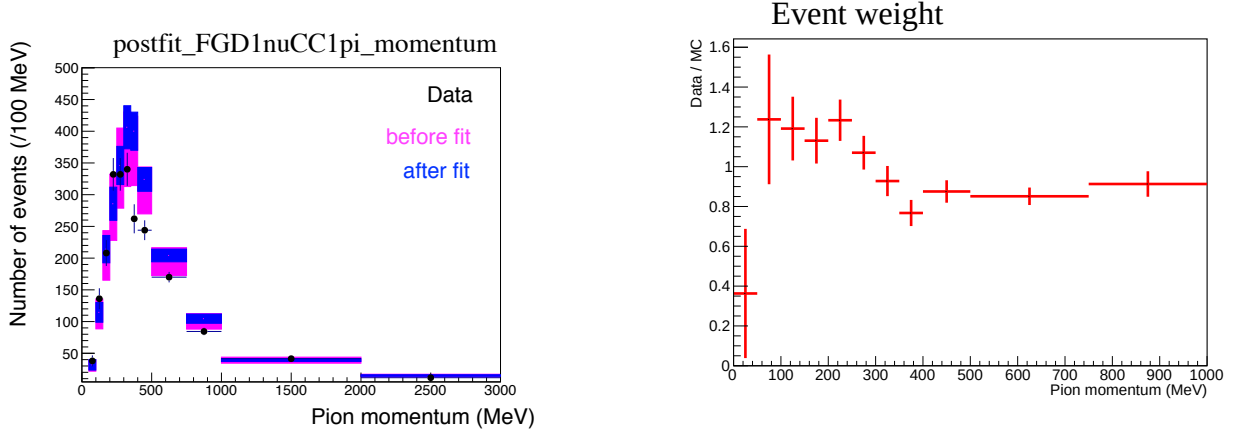
Figure 12.19: Left: Observed pion momentum distribution (black dots), prefit(Magenta) and post-fit(blue) simulated distributions at ND280. Right: The pion momentum ratio between data and the postfit simulation.
