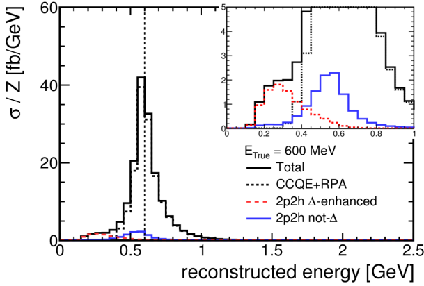
(a) Reconstructed energy dependence of 2p2h
