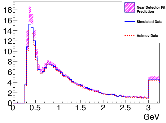
(a) \nu_\mu sample
