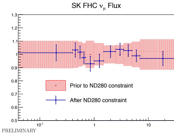
(c) Super-Kamiokande FHC \nu_\mu Flux
