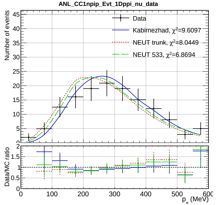
(b) \nu + n \rightarrow \mu + \pi^0 + p
