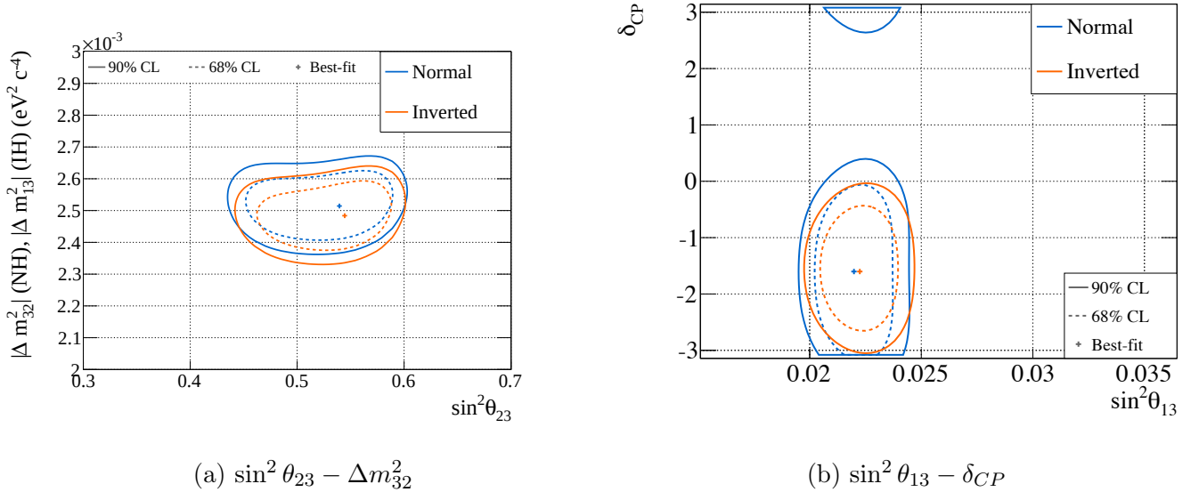
Figure 13.1: Sensitivity for parameter set A with the reactor constraint. The binding energy parameter and the \Delta m_{32}^2 smearing are applied
