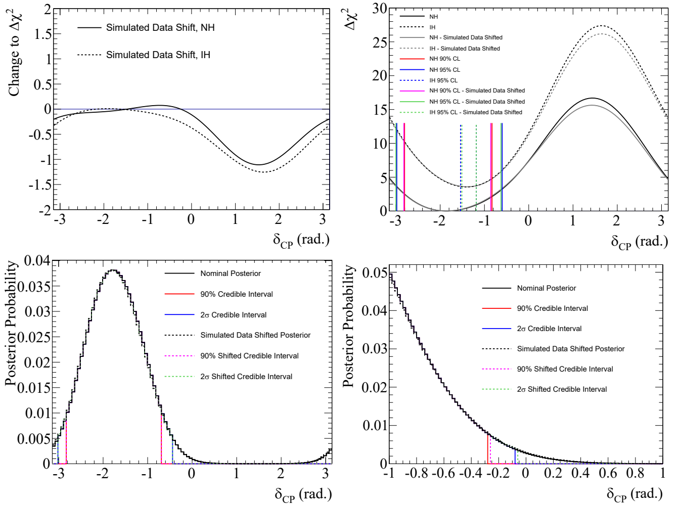
Figure I.13: \Delta\chi^2_{diff}(\delta_{cp}) from the data-driven 1p-1h simulated data study (top left), comparison of the confidence intervals (top right), comparison of credible intervals with a flat prior on \delta_{cp} (bottom left) and comparison of credible intervals with a flat prior on \sin(\delta_{cp}) (bottom right) .
