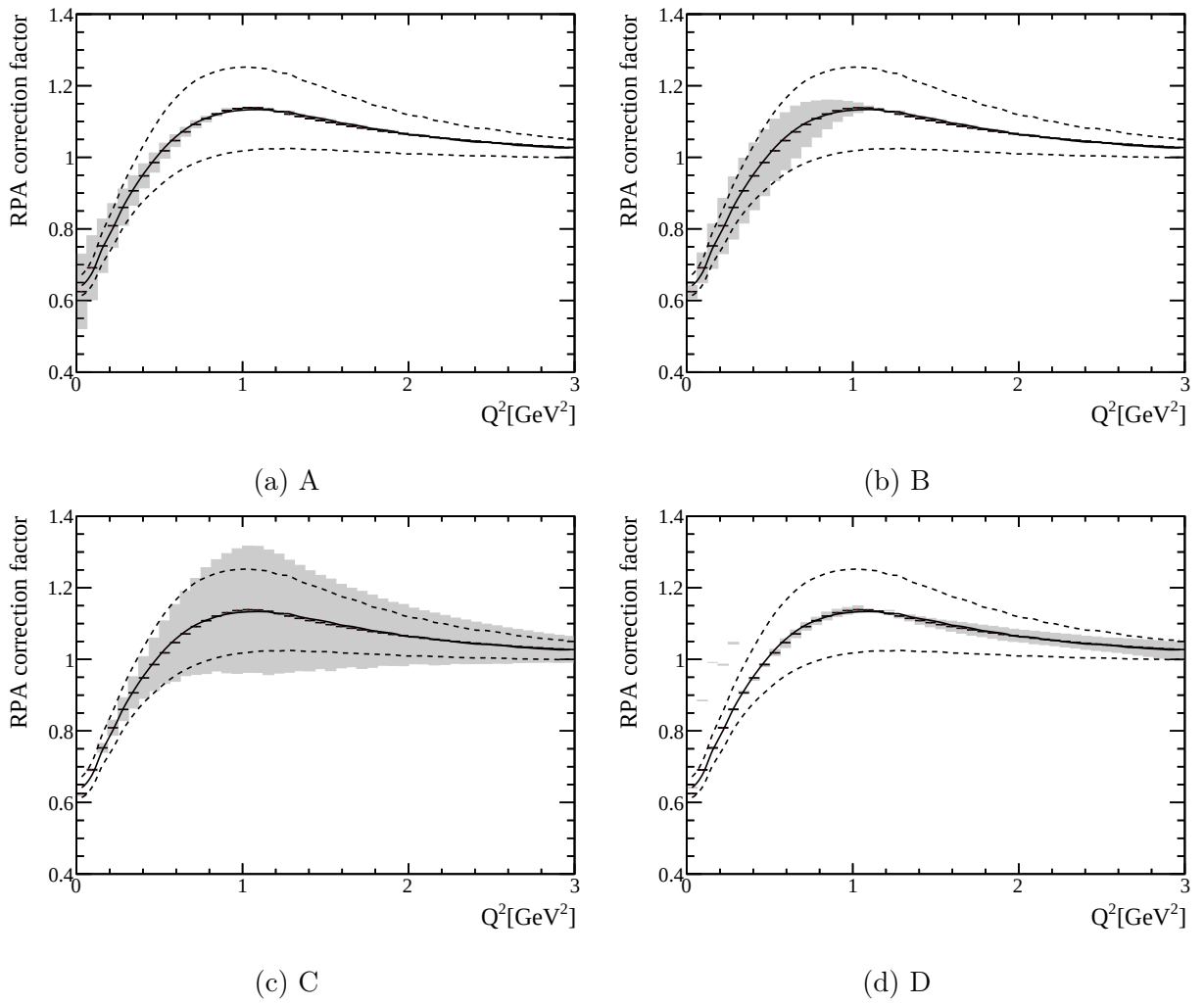
Figure C.1: The 1 \sigma shift of each BeRPA parameter
