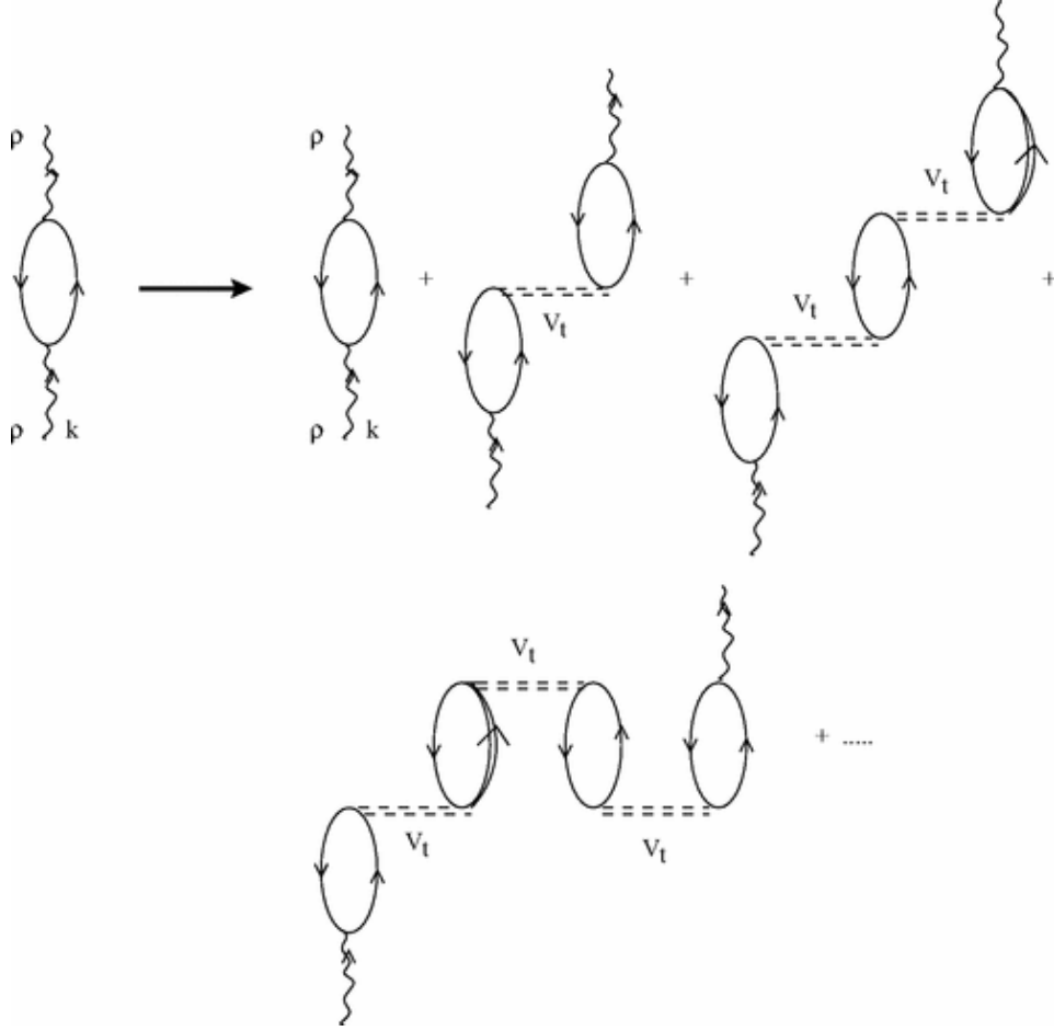
Figure 8.8: Feynman Diagrams of RPA series. Taken from [189].
