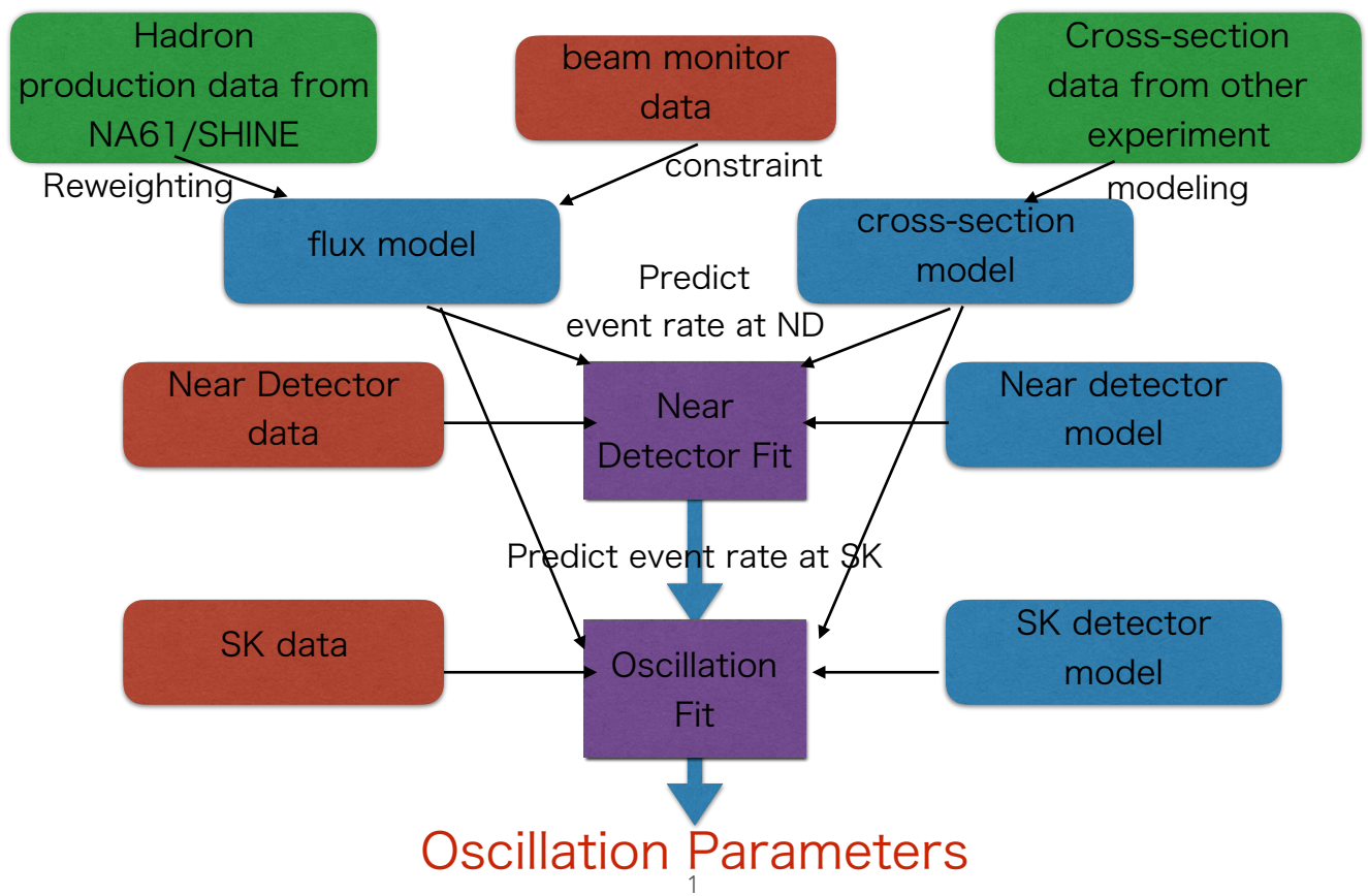
Figure 6.1: Overview of the T2K oscillation analysis
