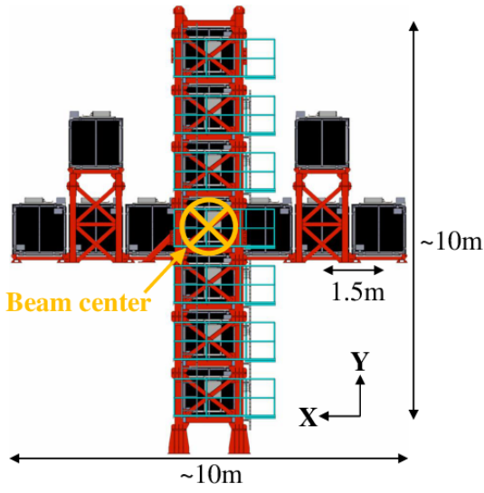
(a) INGRID view from the beam source.
