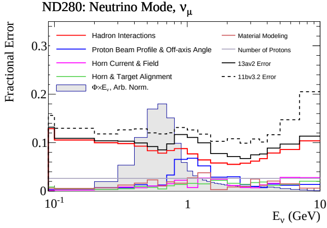
(a) FHC at ND280
