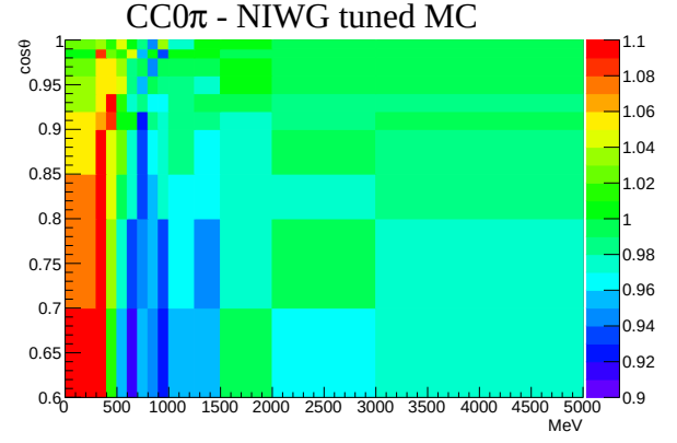
(b) ratio to the nominal model
