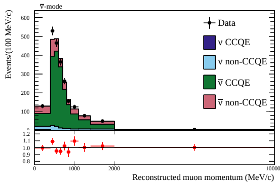
(a) RHC ACC1track momentum distribution
