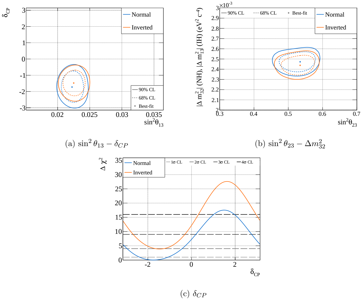
Figure 13.4: The 2D contour for 68% and 90% confidence level and the 1D \Delta \chi^2 surfaces for \delta_{CP} using T2K data and the reactor constraint.
