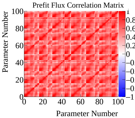
Figure 7.3: ND280 and Super-Kamiokande flux correlation matrix (Left) and covariance matrix(right)
