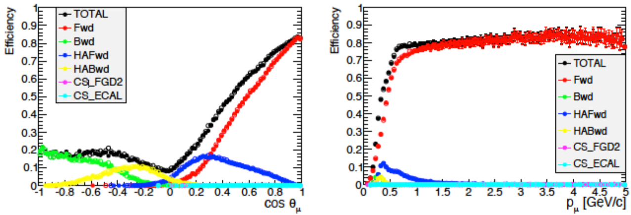
Figure 13.7: Efficiency of the angle and momentum for CC inclusive selection. Red points are for current selection, and yellow, blue and green points are for the improved selections.
