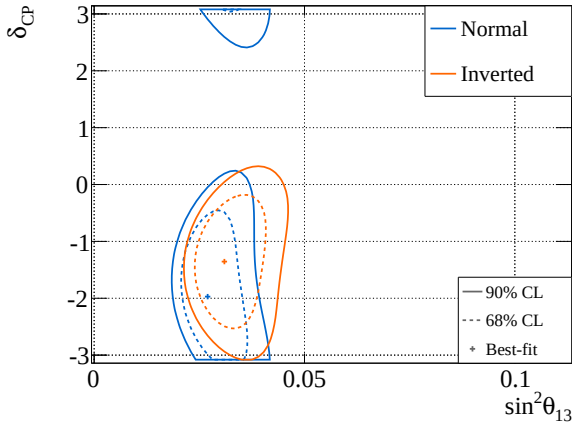
(a) \sin^2 \theta_{13} - \delta_{CP}
