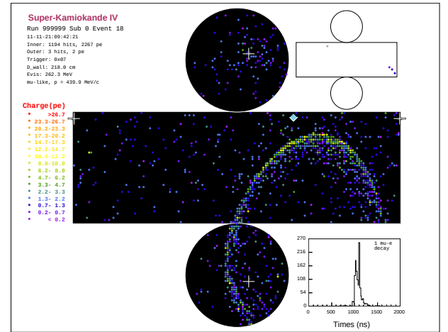
(b) Event display of muon-like ring
