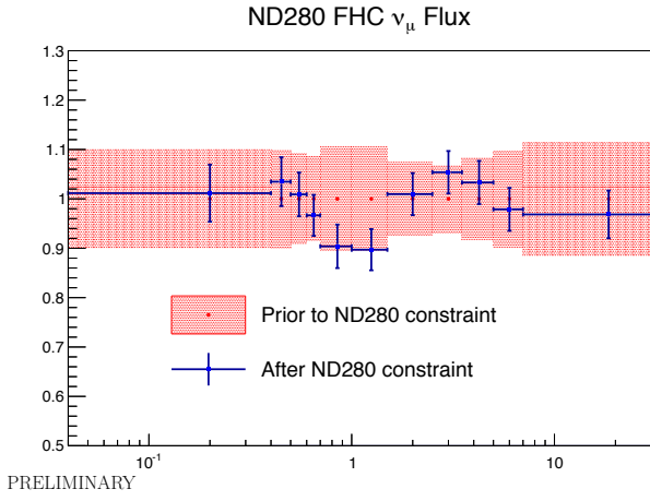
(a) ND280 FHC \nu_\mu Flux
