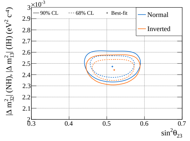
(b) \sin^2 \theta_{23} - \Delta m^2_{32}
