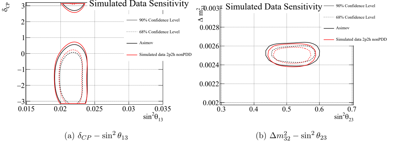
Figure I.11: 2D 68% and 90% contours for Data-driven 2p2h non PDD-like simulated data fits including the reactor constraint on \sin^2 \theta_{13} , assuming normal hierarchy and using the Asimov A oscillation parameter set
