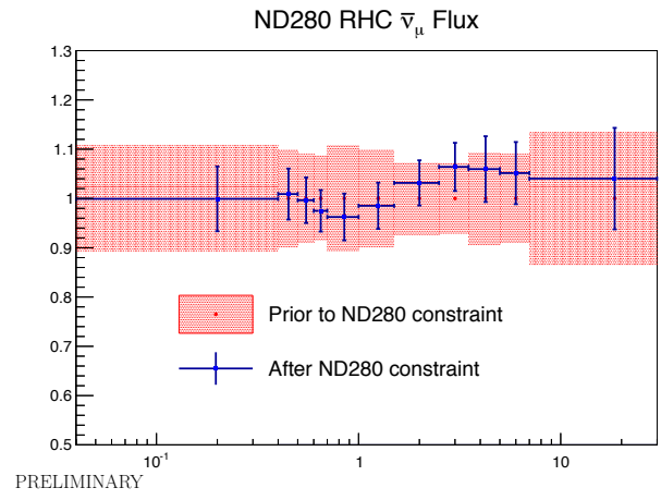
(b) ND280 RHC \bar{\nu}_\mu Flux
