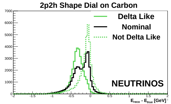
(b) Response of the 2p2h shape parameter
