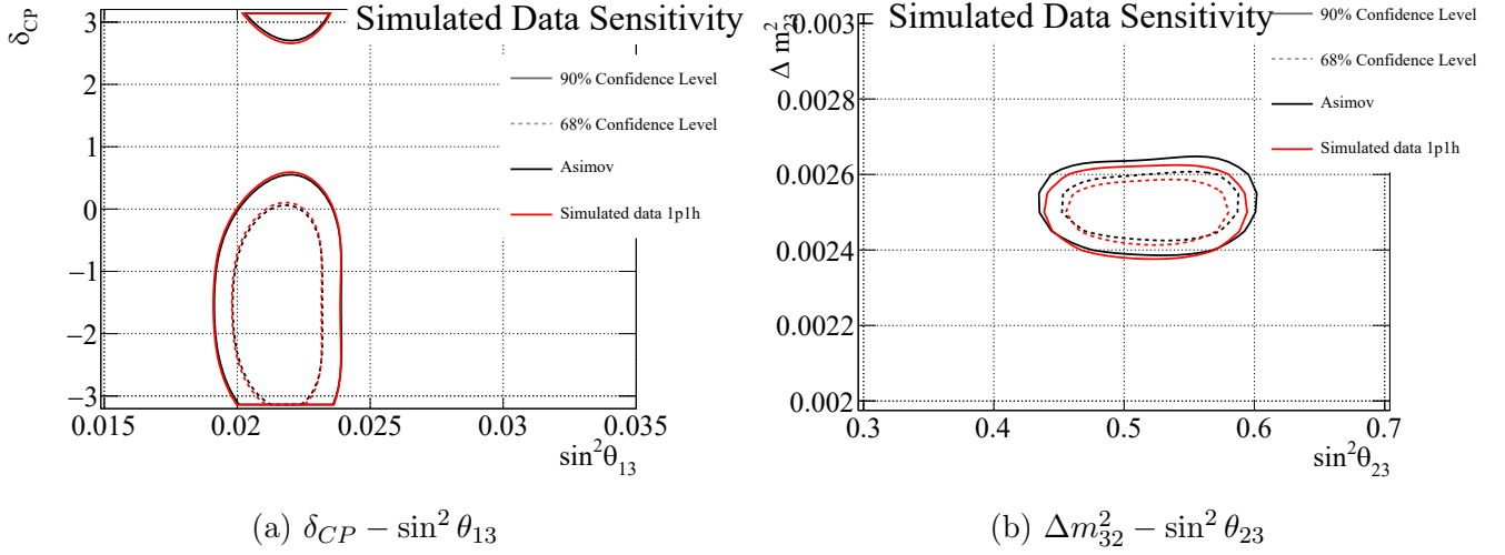
Figure I.3: 2D 68% and 90% contours for Data-driven 1p1h simulated data fits including the reactor constraint on \sin^2 \theta_{13} , assuming normal hierarchy and using the Asimov A oscillation parameter set
