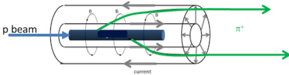
Figure 2.3: Schematic view of the T2K magnetic horn
