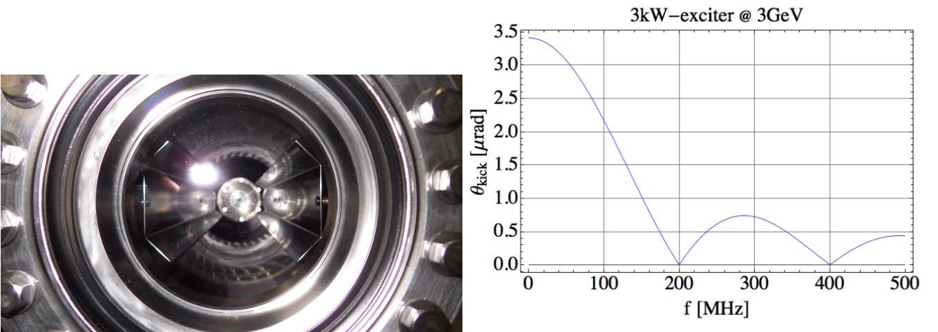
Figure 4.6: Left: Cross-sectional view of stripline kicker, Right: Calculated frequency response of stripline kicker
