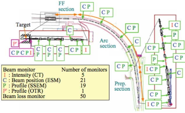
(a) primary beamline
