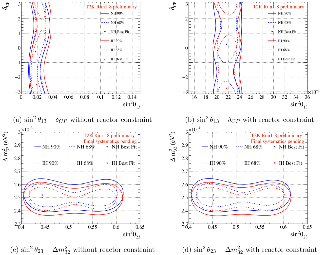
Figure G.1: Sensitivity for Asimov B (2D contours)
