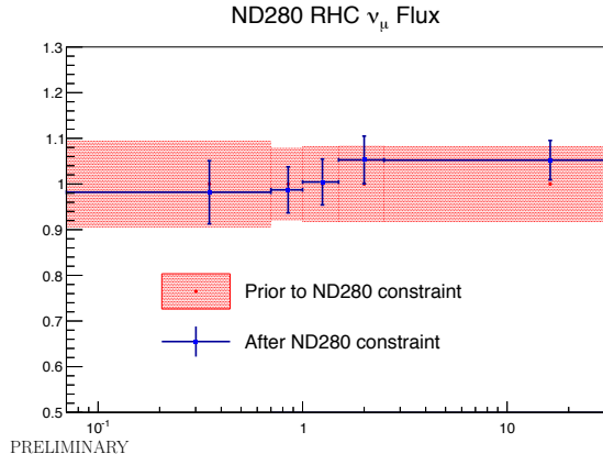
(a) ND280 RHC \nu_\mu flux
