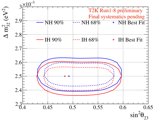
(c) \sin^2 \theta_{23} - \Delta m^2_{32} without reactor constraint
