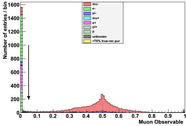
(a) MIP like track
