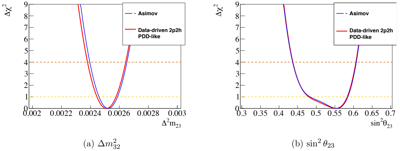
Figure 12.17: The 1D sensitivity curves of the \sin^2 \theta_{23} and \Delta m_{32}^2 for the data-driven 2p2h PDD-like simulated data fit and Asimov data fit.
