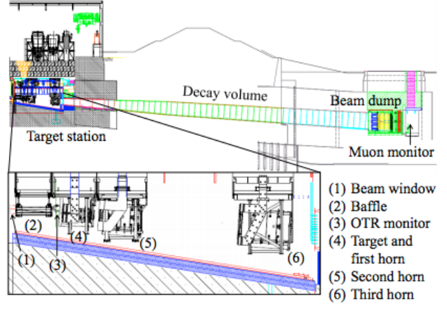
(b) secondary beamline
