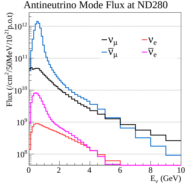
(b) RHC at ND280
