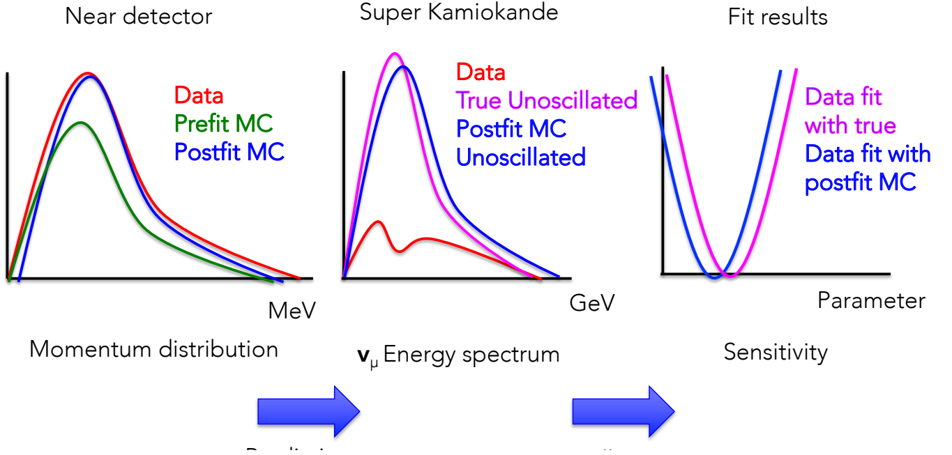
Figure 12.1: The schematic view of the fitting bias due to a wrong model
