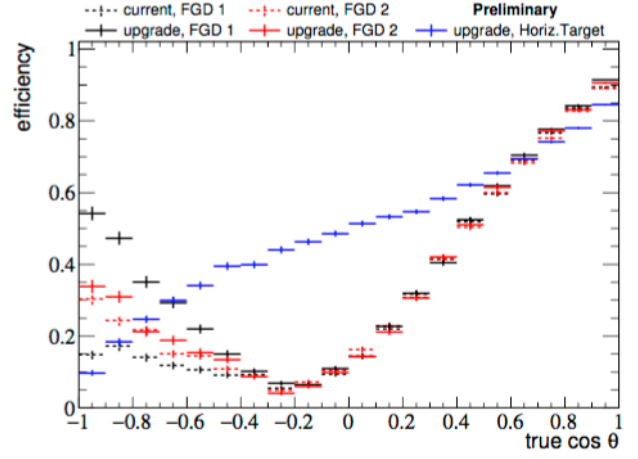
(b) Estimated angle efficiency of the ND280 upgrade detector (Black) comparing current FGD measurements.
