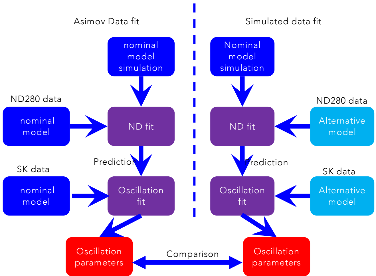
Figure 12.2: Procedure of simulated data study
