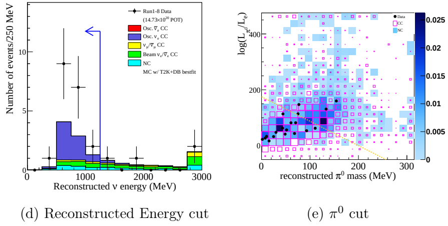
Figure 10.5: Cut criteria for \nu_e 1 decay electron samples
