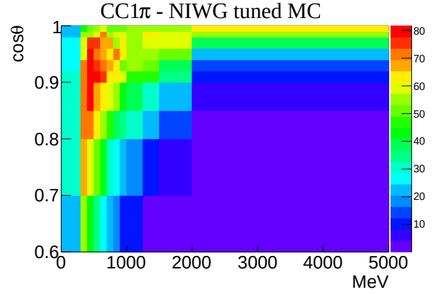
(b) CC1 \pi
