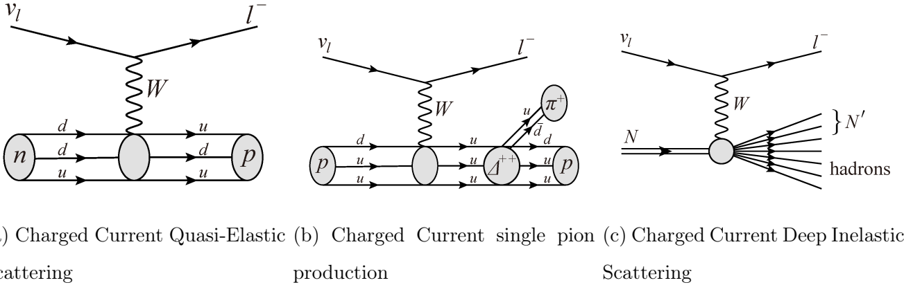
Figure 8.3: Feynmann diagrams of Charged Current neutrino-nucleon interaction
