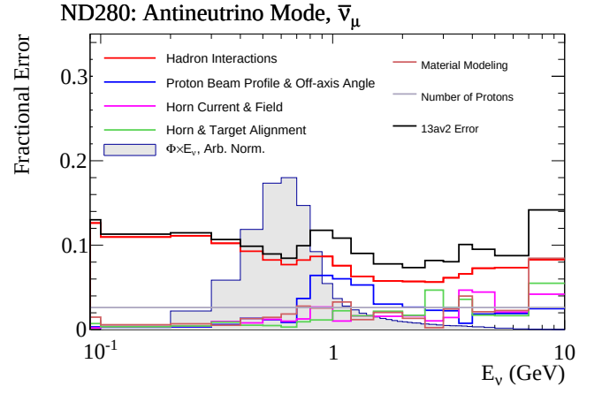
(b) RHC at ND280
