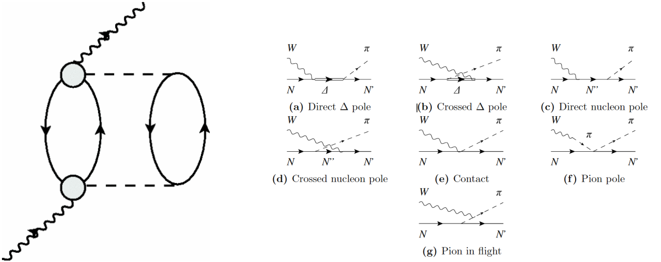
Figure 8.10: Left: W self energy of 2p2h. Wave lines correspond to W, solid lines correspond to nucleons and dashed lines correspond to pions. Right: Contributions in the circle in the left plot. Taken from [189].
