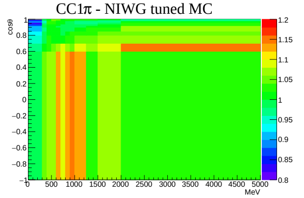
(b) CC1 \pi
