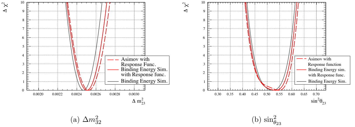
Figure 12.23: The 1D sensitivity curves of \Delta m_{32}^2 , \sin^2\theta_{23} for Asimov (dashed red) and the binding energy simulated data with (solid red) and without (Solid black) the binding energy parameter.
