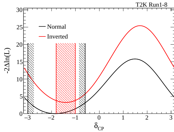
Figure 13.5: 1D \Delta \chi^2 distribution as a function of \delta_{CP} of the data fit the with reactor constraint and 2\sigma interval calculated with the Feldman-Cousins method.
