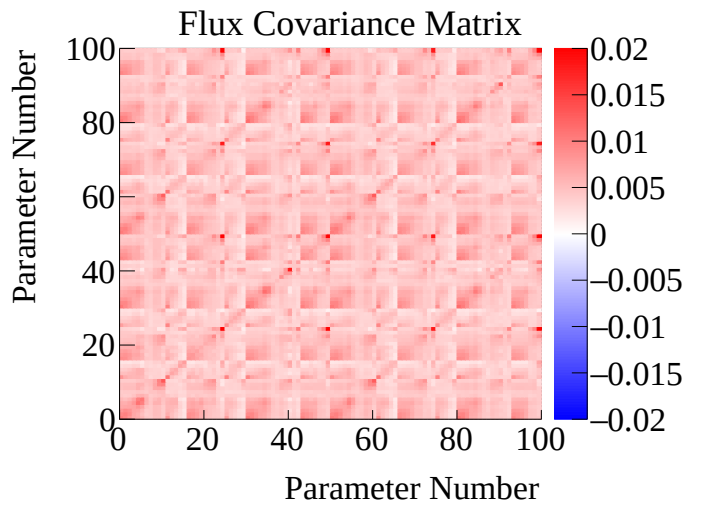
Figure 7.3: ND280 and Super-Kamiokande flux correlation matrix (Left) and covariance matrix(right)
