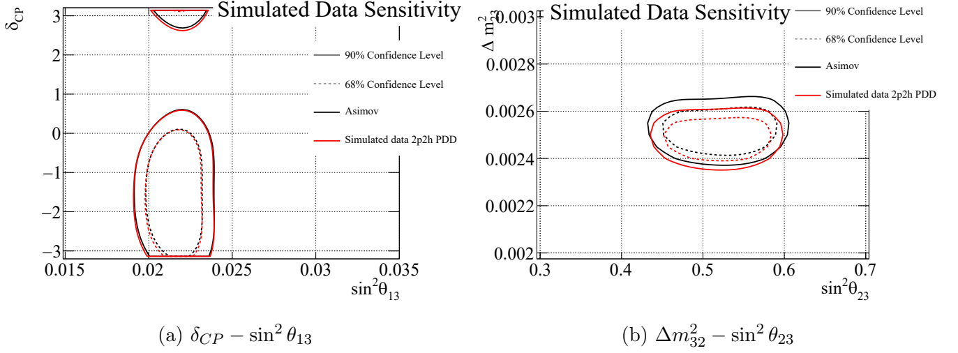
Figure I.7: 2D 68% and 90% contours for Data-driven 2p2h PDD-like simulated data fits including the reactor constraint on \sin^2 \theta_{13} , assuming normal hierarchy and using the Asimov A oscillation parameter set
