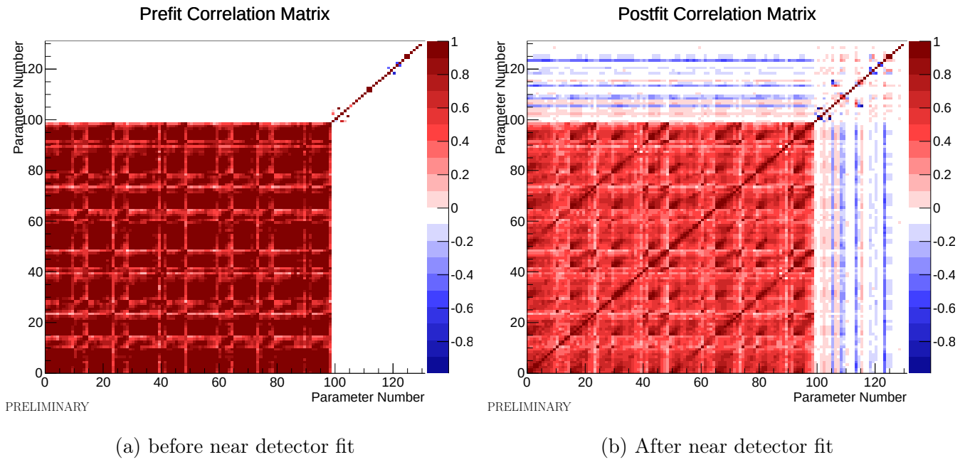
Figure 9.11: Correlation matrix for the cross-section and flux parameters before and after the near detector fit. The 0-99 bin corresponds to flux parameters, 100-131 bin corresponds to cross-section parameters.
