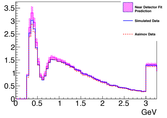
(b) \bar{\nu}_\mu sample
