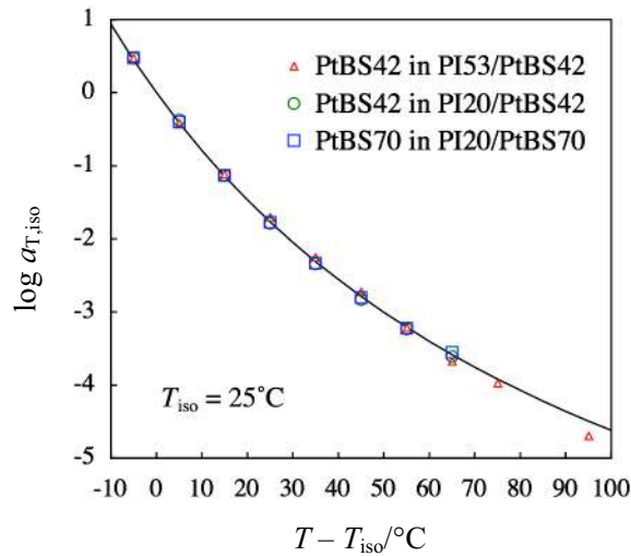
Fig. 7-16: Shift factor a_{T,\text{iso}} defined with respect to the iso- \tau_s temperature T_{\text{iso}} = 25^\circ\text{C} for PtBS in the PI53/PtBS42 (Figure 7-15), PI20/PtBS42, and PI20/PtBS70 blends. All these blends have the same PI content, w_{\text{PI}} = 55.7\text{ wt\%} . The solid curve indicates the WLF equation for PtBS bulk with T_{r,\text{bulk}} = 180^\circ\text{C} .
