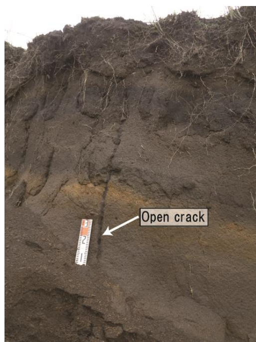
Fig. 13 An open crack filled with BI at the scarp of landslide KGC-2-1. This crack must have been made before the 2016 event.
