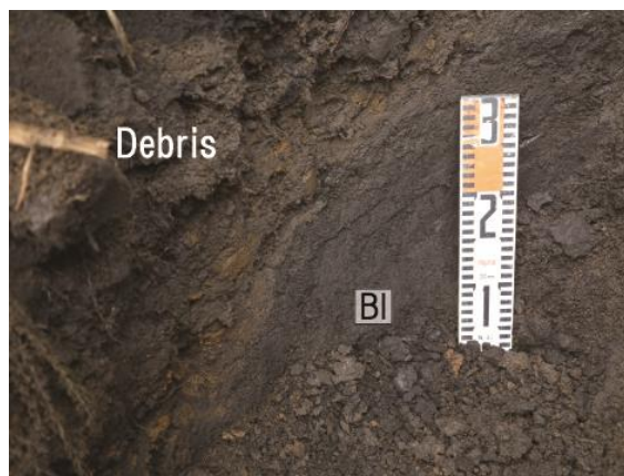
Fig. 15 A sliding surface formed in BI layer with high water content (KGC-3).
