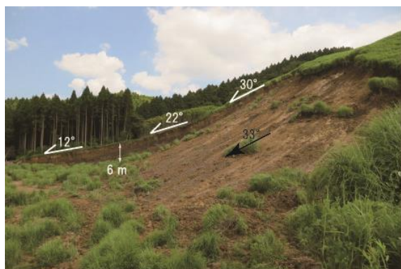
Fig. 25 Oblique view of landslide AVL-3. Surface slope angles changed from 30° in higher elevations to 12° in lower. A sliding surface of Br with lava blocks was widely exposed.
