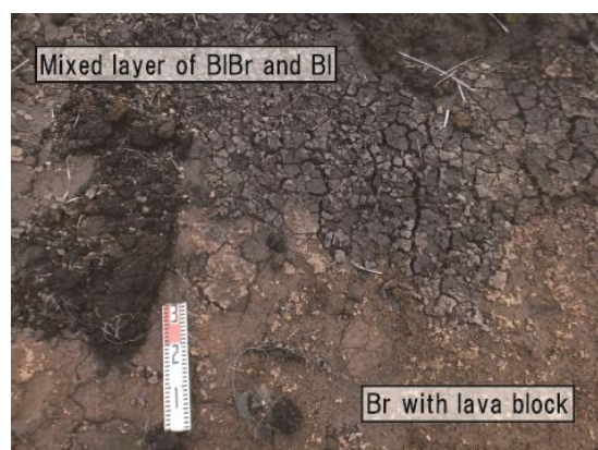
Fig. 12 A sliding surface formed in the base of the mixed layer of BI Br and BI in KGC-2-1
