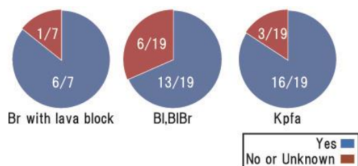
Fig. 44 Diagram showing whether the slid layers were undercut or not before the landslide. Each circle represents each sliding surface material.
