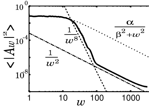
Figure 6. Power spectrum. In an intermediate range of frequency, we found different fluctuations from the Lorentzian. \alpha = 12.69 , \beta = 13.61 . The lines \frac{1}{\omega^2} and \frac{1}{\omega^8} are shown for the sake of comparison.
