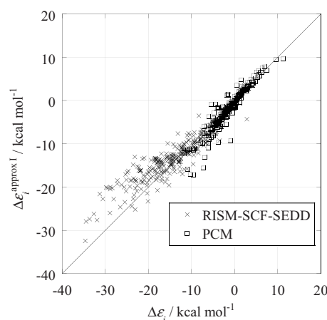
FIG. 6. Comparison between the exact values ( \Delta\epsilon_i ) and the approximation formula of Eq. (15).
