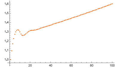
Figure 2: DDE Split Solution \tau = 0.1
