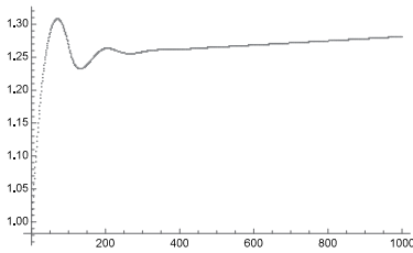
Figure 1: DDE Split Solution \tau = 0.01
