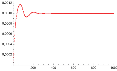
Figure 4: Relative Error DDE Split \tau = 0.01
