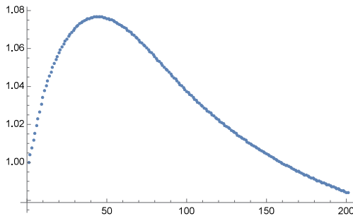
Figure 3: Case2 DDE Split Solution \tau = 0.01
