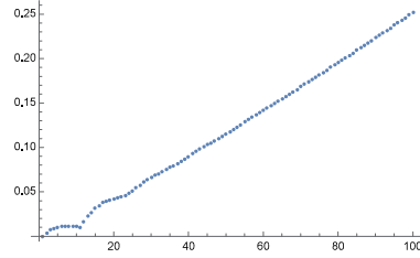
Figure 5: Relative Error DDE Split \tau = 0.1
