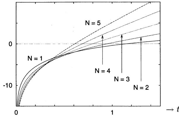
Fig. 1. Errors in the case of the 2-stage method (3.1)
