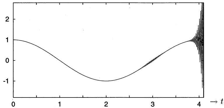
Fig. 2. Approximate solution in the case of the 3-stage method (3.3) for N = 200
