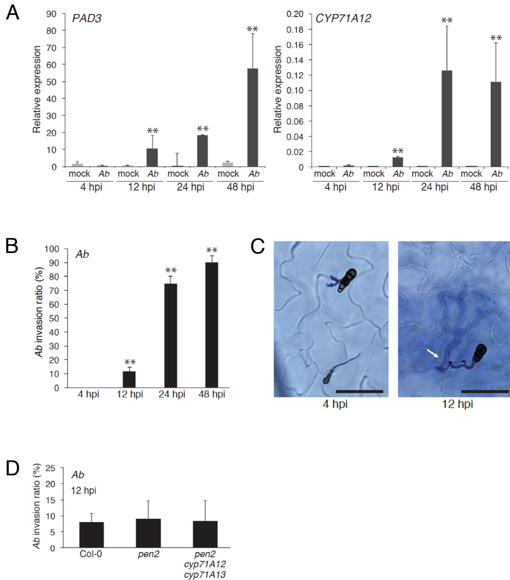
Fig. II-2. The invasion of Ab activates the expression of PAD3 and CYP71A12 .
