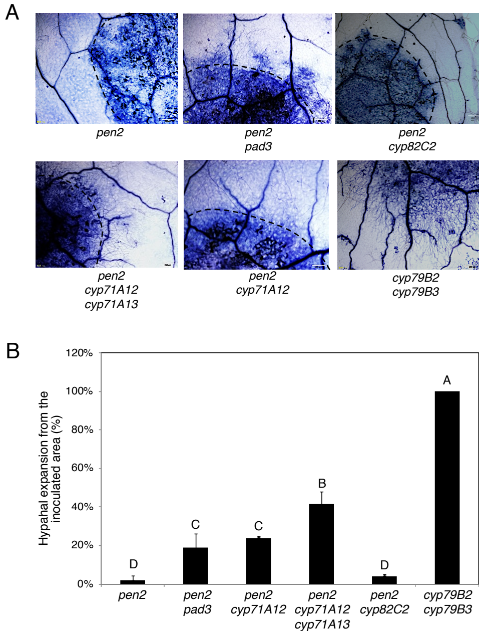
Fig. I-3. Trp-derived secondary metabolites, camalexin and ICAs, are required for postinvasive defense against Ctro .
