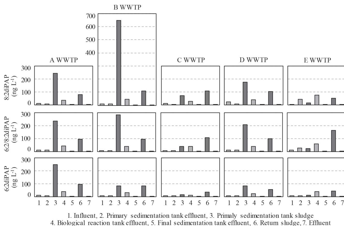
Fig. 5 Concentrations of 3 diPAPs (6:2diPAP, 6:2/8:2diPAP, 8:2diPAP) in wastewater treatment plants.
