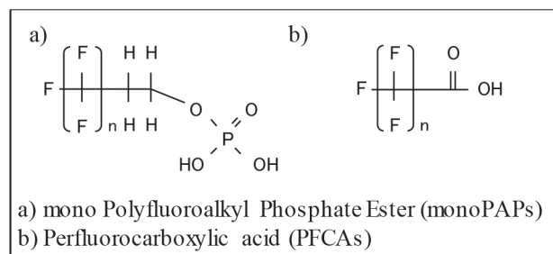
Fig. 1 Chemical structure of PAPs and PFCAs.
