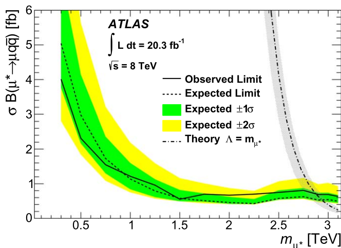
Figure 3. Limit at 95% CL on cross section times branching ratio \sigma(pp \rightarrow \mu\mu^*)B(\mu^* \rightarrow \mu q \bar{q}) as a function of the \mu^* mass, where q is any quark except the top quark. The solid line is the limit and the dotted line is the expected limit. The theoretical \sigma B for the limiting case \Lambda = m_{\mu^*} along with its uncertainties is also shown.
