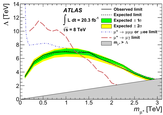
Figure 4. Limit at 95% CL on the compositeness scale \Lambda as a function of the \mu^* mass. The solid line is the observed limit, and the short dashed line is the expected limit. Also indicated are previous results from ATLAS based on \mu^* \rightarrow \mu\gamma (long dashed line) and \mu^* \rightarrow \mu\ell\ell (dotted–dashed line), where \ell is an electron or muon.
