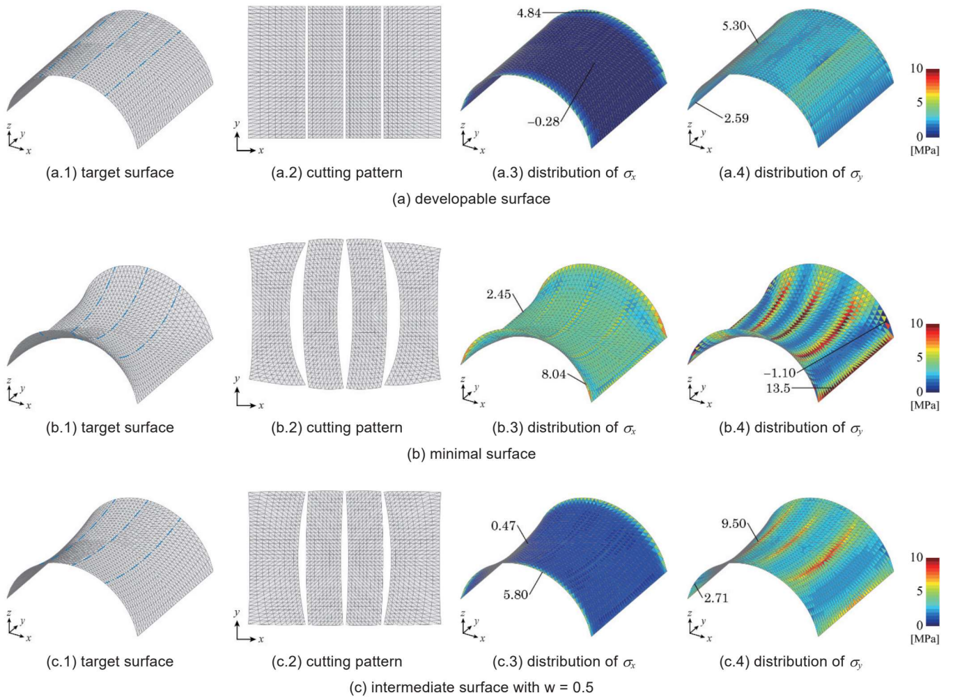
Fig. 6 Surfaces generated with cutting pattern 2 ( m = 4 ) and h = 2.0 m
