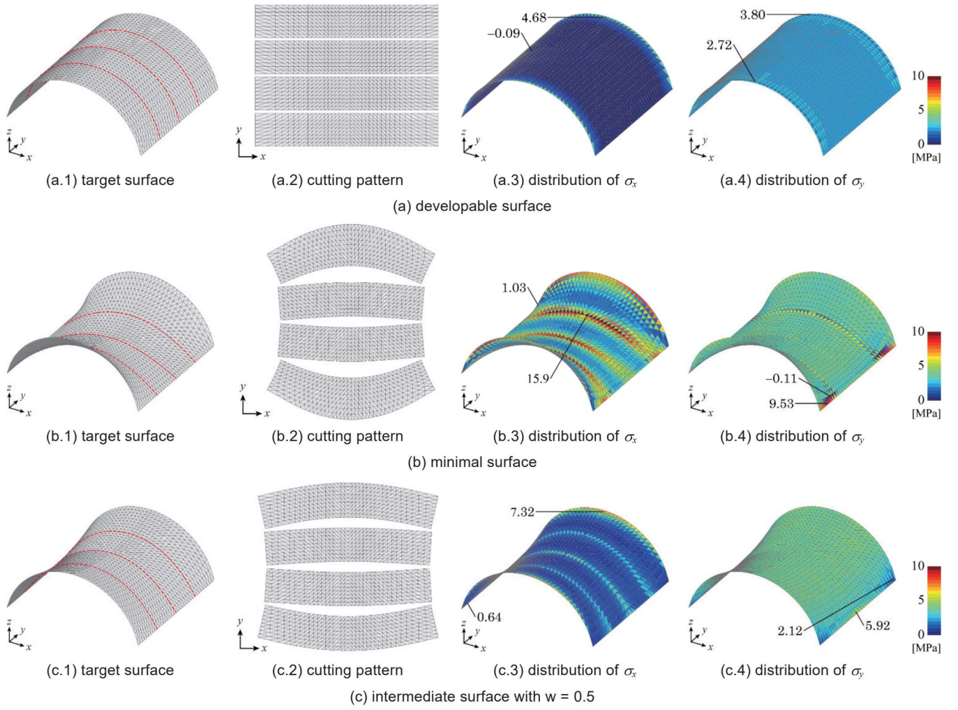
Fig. 5 Surfaces generated with cutting pattern 1 ( m = 4 ) and h = 2.0 m
