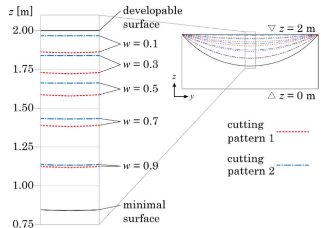
Fig. 7 Elevations of target surfaces ( h=2.0 m)
