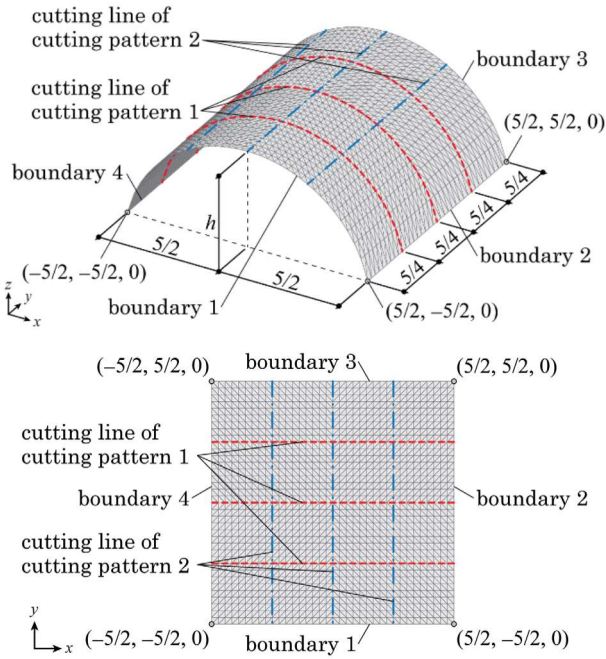
Fig. 3 Initial shape with cylindrical boundary (unit: m)
