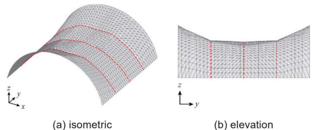
Fig. 4 Intermediate surface generated with area constraint ( h=2.0 m, w=0.5 )
