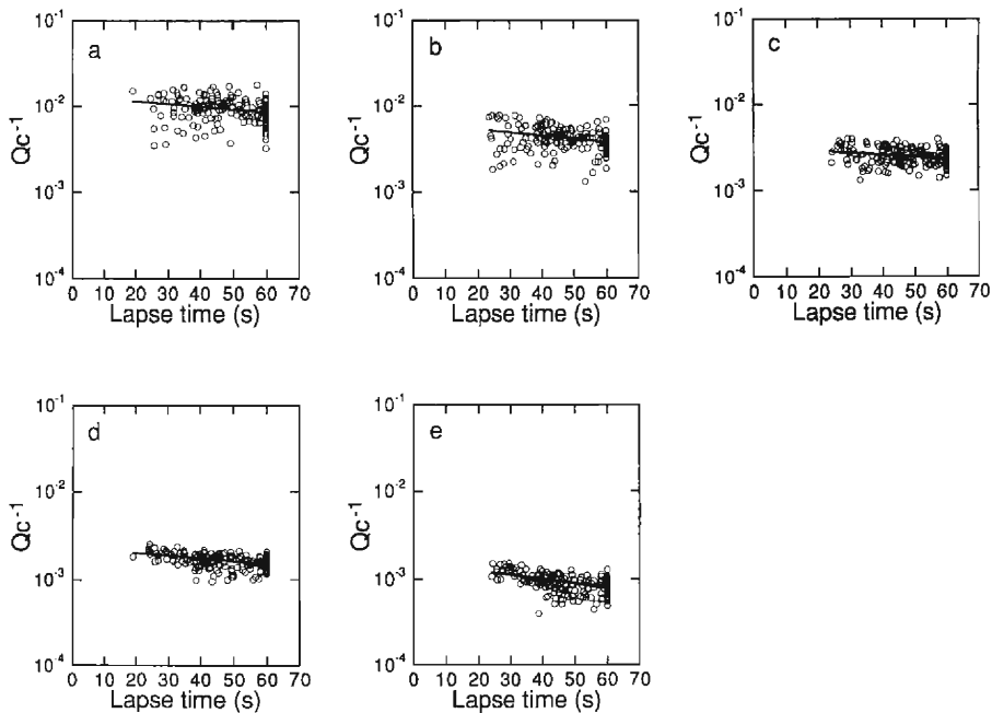
Fig. 15. (a), (b), (c), (d) and (e) indicate distribution of coda Q^{-1} versus lapse time in the volcanic area at 1.5, 3.0, 6.0, 12.0 and 24.0 Hz, respectively. Solid line is linear trend fitted by the least squares method.
