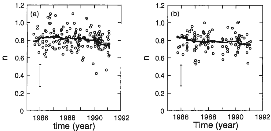
Fig. 8. (a) and (b) indicate temporal variations in the power of frequency n for coda Q^{-1} in the volcanic and the tectonic areas, respectively. Solid curve is running mean of 21 successive data and solid bars show standard deviation from the running mean.
