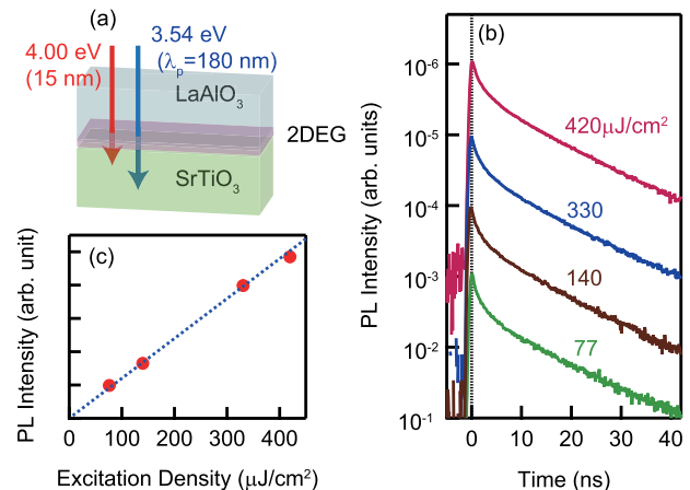
FIG. 2. (a) Schematic illustration of the probing depth for the different excitation energy values. (b) PL dynamics of the LAO/STO heterostructure under different excitation intensities. Excitation photon energy was 4.00 eV. (c) Excitation-density dependence of the time-integrated PL intensity.
