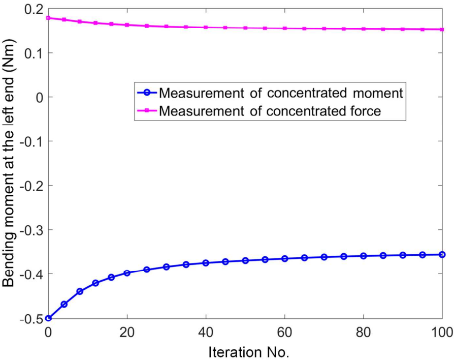
Fig. 4 Convergence of bending moment at left end of propped cantilever beam 203x155mm (192 x 192 DPI)
