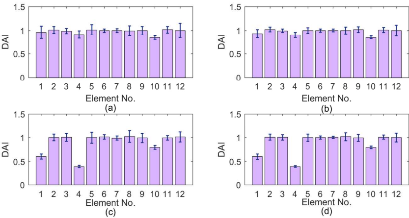
Fig. 8 Mean values and standard deviations of DAI with 0.1mm noise for: (a) small damage case D1 by min-CRE approach, (b) small damage case D1 by modified min-CRE approach, (c) large damage case D2 by min-CRE approach, (d) large damage case D2 by modified min-CRE approach.
