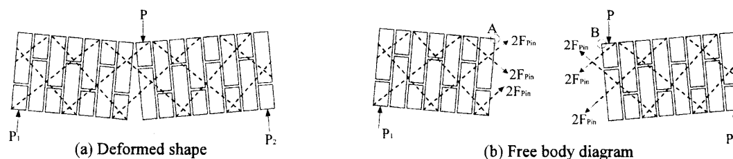
Figure 3 Failure Mode 1
