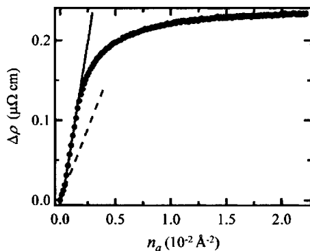
FIG. 10. The change in film resistivity \Delta\rho as a function of \text{C}_{60} coverage for a 20-nm-thick Cu film. The resistivity-decrease effect by the formation of a conducting \text{C}_{60} monolayer is subtracted and the change due only to the increase in the surface scattering of conduction electrons is shown. The straight lines indicate the slopes of the change in resistivity.
