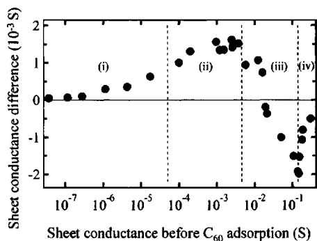
FIG. 1. Change in the sheet conductance of a C_{60} /Au bilayer film. The vertical axis represents the differences in sheet conductances before and after C_{60} deposition. The change has four stages with respect to the conductances of Au underlayers, i.e., with respect to the degree of underlayer metal growth.
