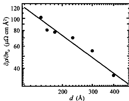
FIG. 7. The initial slope of the change in resistivity, \partial \rho / \partial n_a (n_a \rightarrow 0) , vs the film thickness of Au films, d , plot. The straight line is a regression fit with a slope of -1 .
