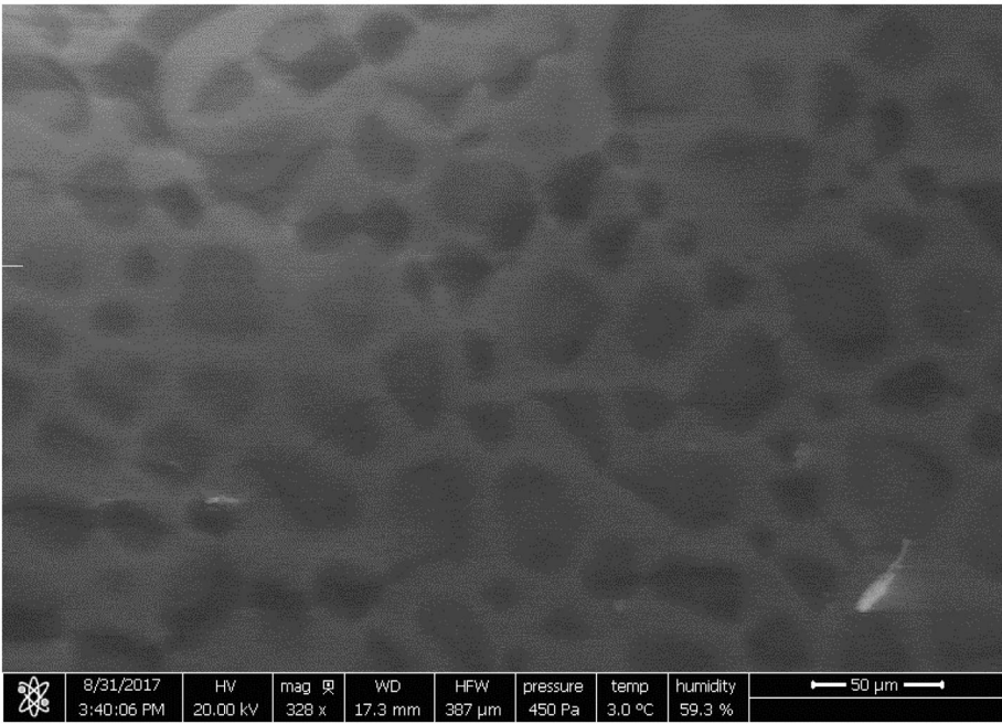
Figure 1. SEM picture of silk-elastin sponge. Note: Silk-elastin sponge E (density, 25 mg/cm 3 ; thickness, 1.25 mm).
