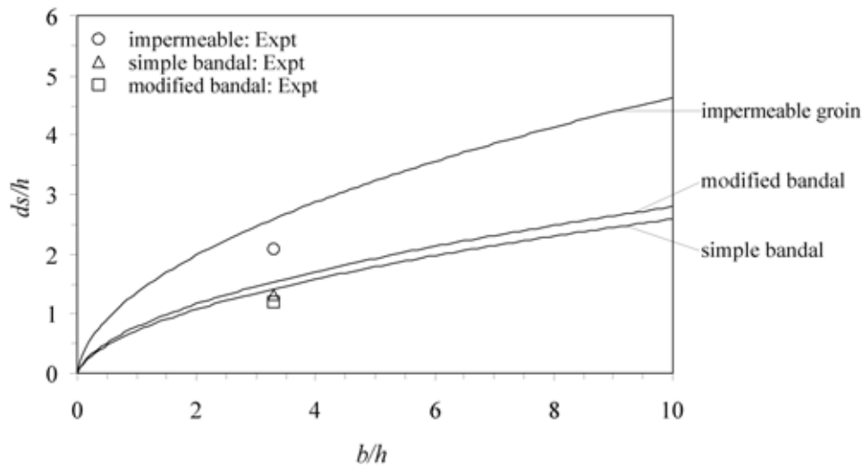
Fig. 12 Prediction of local scour depth
