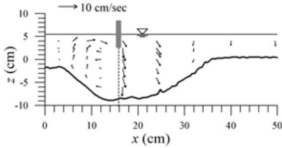
Fig. 8 Velocity vectors ( u_x , u_z ) at the end of the first bandal (section BT-BT of figure 3): simple bandal case
