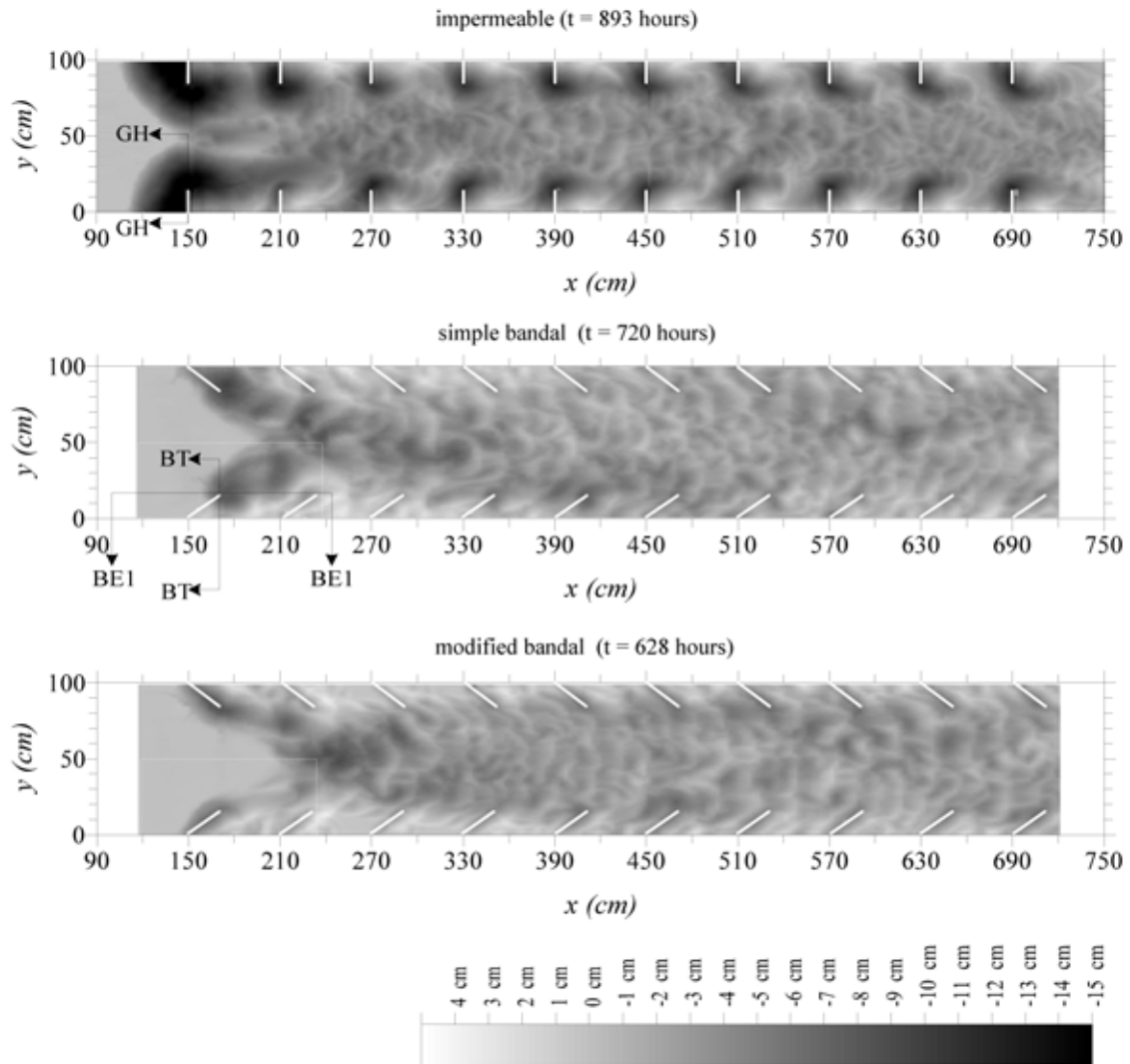
Fig. 3 Final bed shape for impermeable groins, simple bandals and modified bandals
