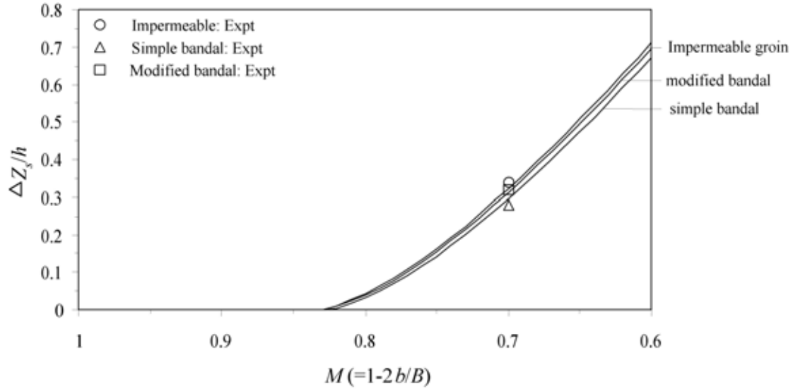
Fig. 11 Comparison of main channel degradation for impermeable groins and bandals (both prediction lines and experimental data are for u*/u_{*c} = 0.83 )
