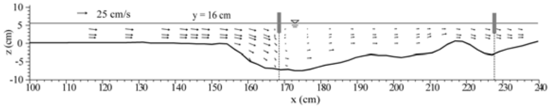
Fig. 5 Vectors ( u_x, u_z ) along BE1-BE1 in figure 3 for simple bandals
