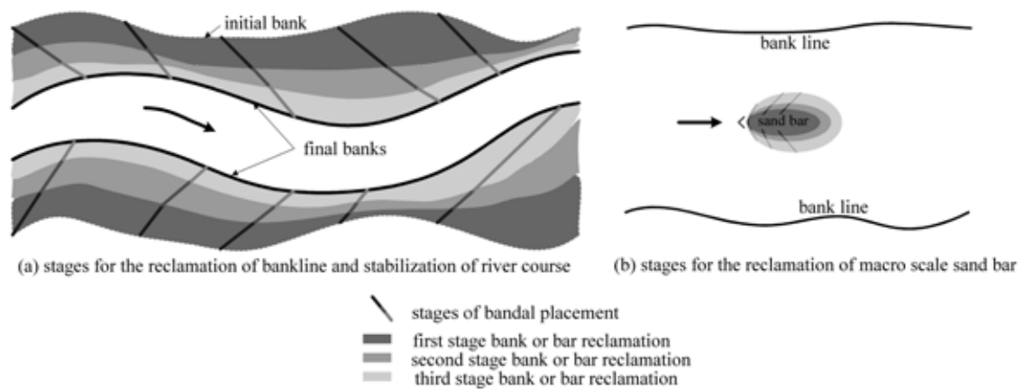
Fig. 13 Schematic sketch for river course and sand bar stabilization using bandals
