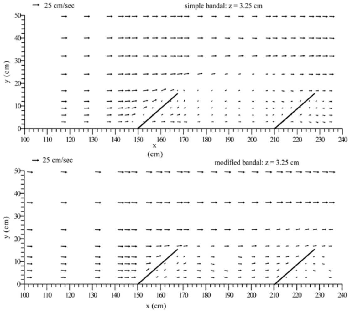
Fig. 6 Velocity vectors ( u_x, u_y ) near the water surface around first two structures for both the simple and modified bandal cases
