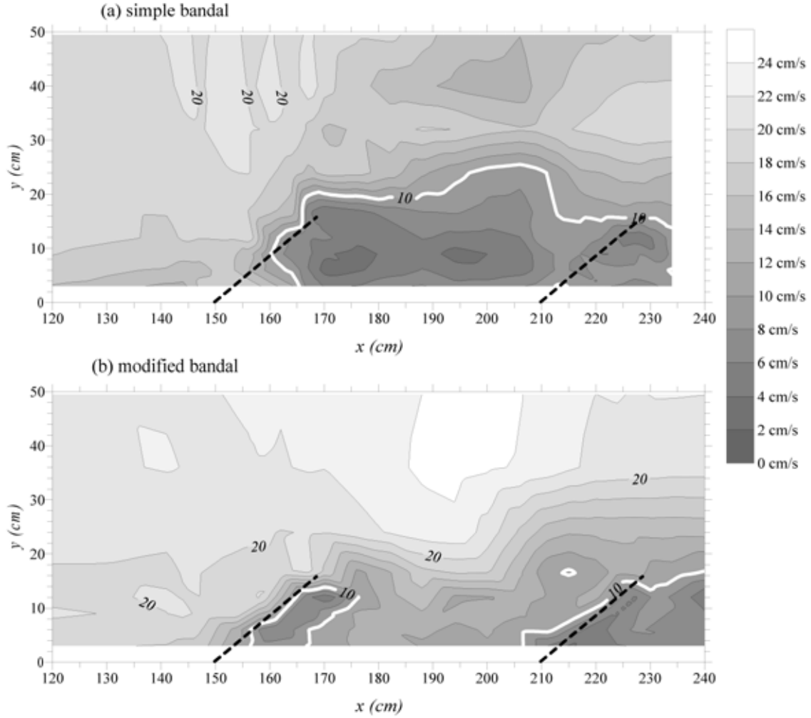
Fig. 4 Depth average isovels ( u_x , u_y , u_z ) around bandal fields and main channel for both simple and modified bandals
