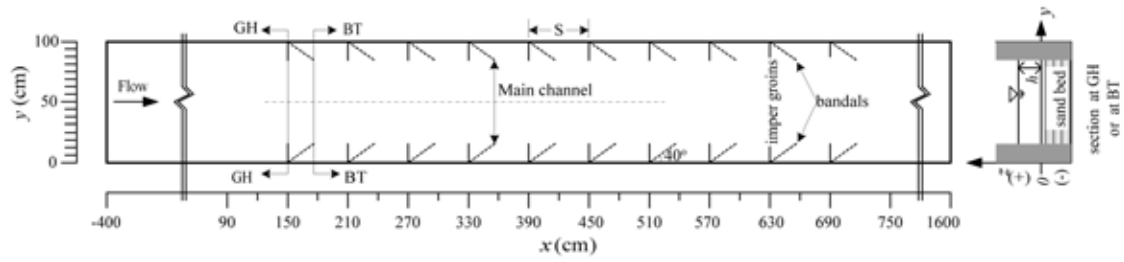
Fig. 2 Experimental arrangements
