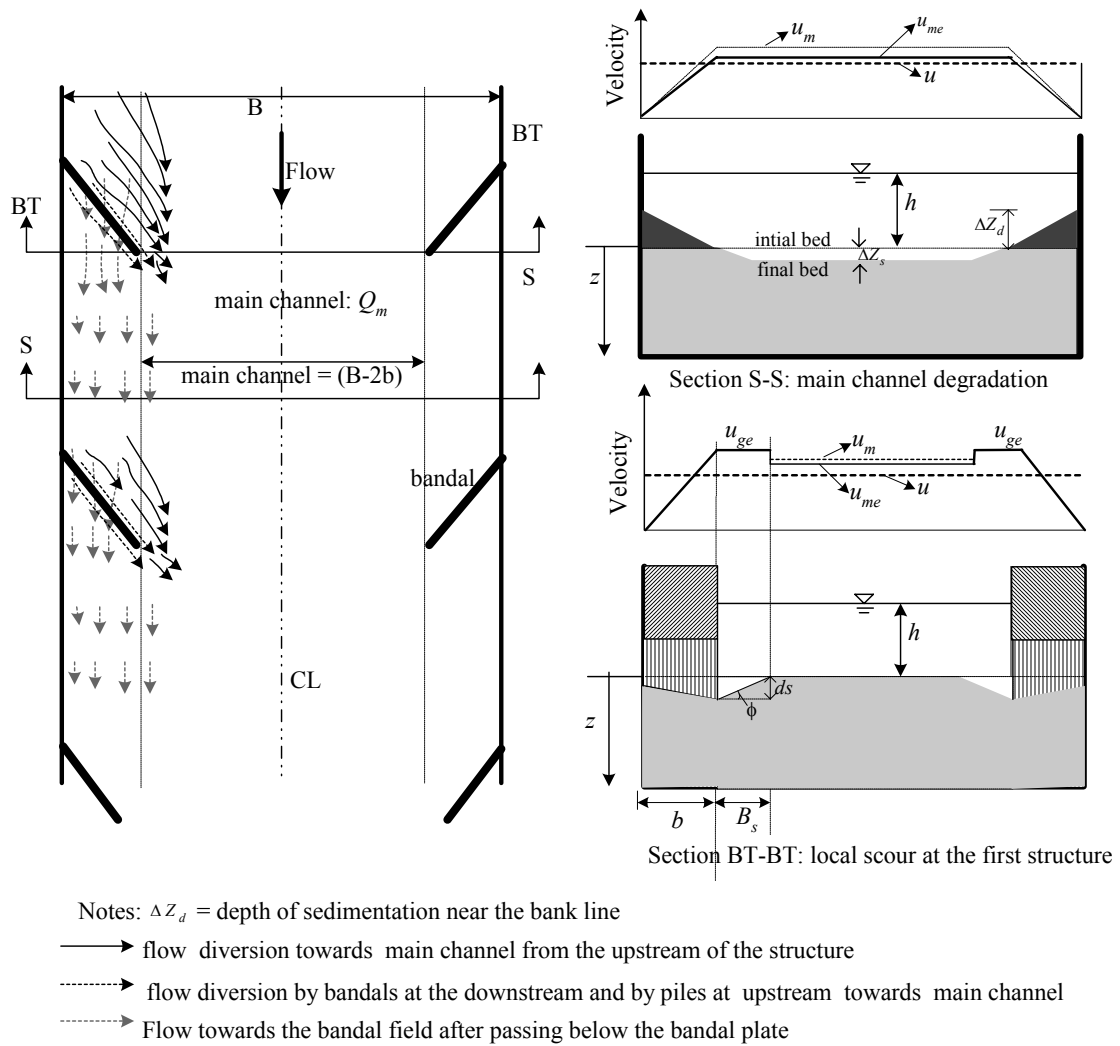
Fig. 10 Definition sketch for bed degradation and local scour model
