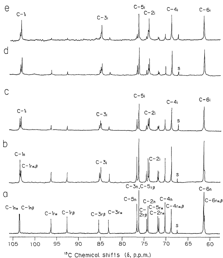
Fig. 5 13 C-N.M.R. spectra of the laminari-oligosaccharides at 25°C in deuterium oxide: laminaribiose (a), laminaritriose (b), laminaritetraose (c), laminaripentaose (d), and laminariheptaose (e). Symbols: dioxane (s), reducing end residue (r), internal residues (i), and non-reducing end residue (n).
