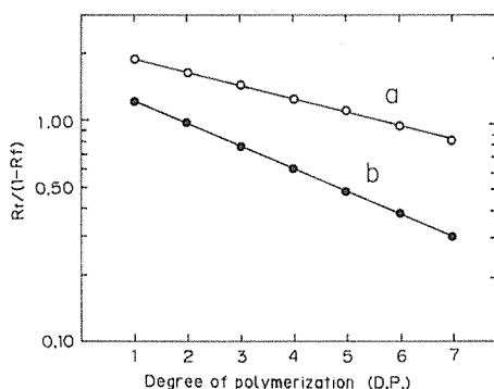
Fig. 7 Relation between R_f/(1-R_f) and degree of polymerization of laminari-oligosaccharides: The R_f values were obtained by T. L. C. using (a) 1-butanol-2-propanol-water (3:12:4, v/v) (○) and (b) 1-butanol-ethanol-water (5:3:2, v/v) (●).
