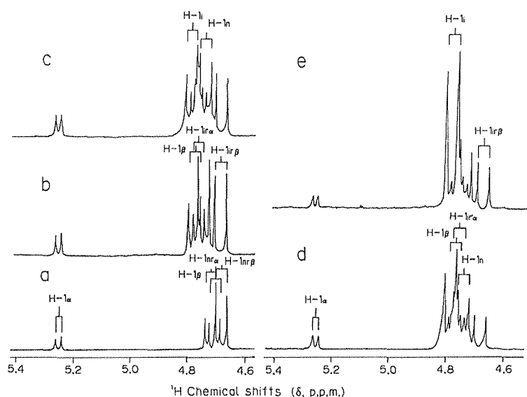
Fig. 6 ^1\text{H} -N.M.R. spectra of laminari-oligosaccharides at anomeric region at 80^\circ\text{C} in deuterium oxide: laminaribiose (a), laminaritriose (b), laminaritetraose (c), laminaripentaose (d), and laminariheptaose (e). Symbols: anomeric protons of the reducing end ( \text{H-1}_\alpha , \text{H-1}_\beta ), internal and adjacent to the reducing end ( \text{H-1}_{r\alpha} , \text{H-1}_{r\beta} ), internal ( \text{H-1}_i ), non-reducing and adjacent to the reducing end ( \text{H-1}_{n\alpha} , \text{H-1}_{n\beta} ), and non-reducing end ( \text{H-1}_n ) glucose residues.
