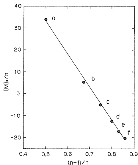
Fig. 8 Relation between [M]_0/n and (n-1)/n , where [M] and n were molar optical rotation and degree of polymerization, respectively: laminaribiose (a), laminaritriose (b), laminaritetraose (c), laminaripentaose (d), laminarihexaose (e), and laminariheptaose (f).
