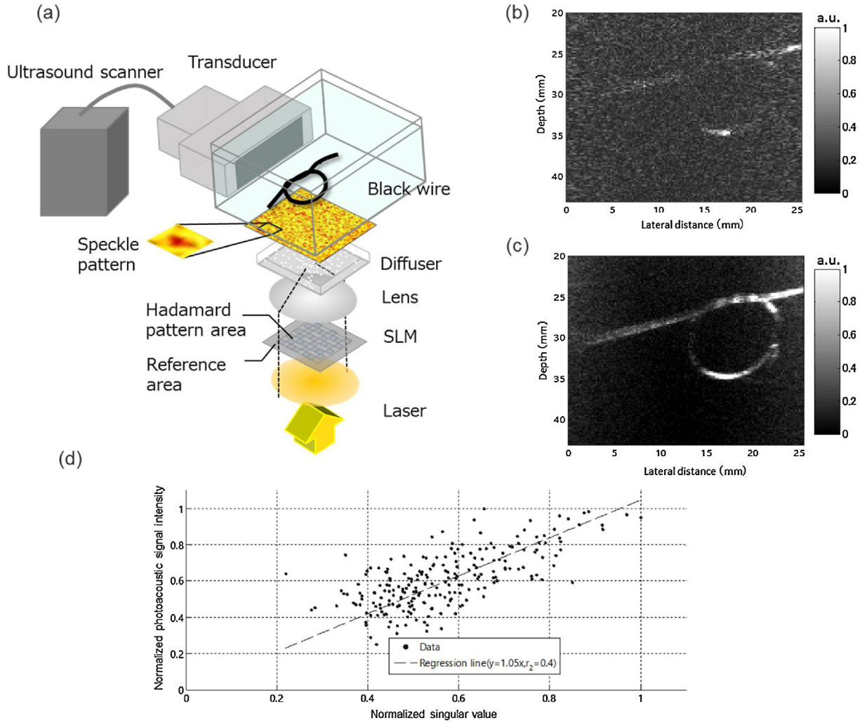
Fig. 4. Experiment results of a wire phantom illuminated with 8 \times 8 Hadamard modulated light.
