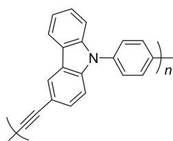
Chart 2. Structure of Poly(3,9-carbazolyleneethynylene)
