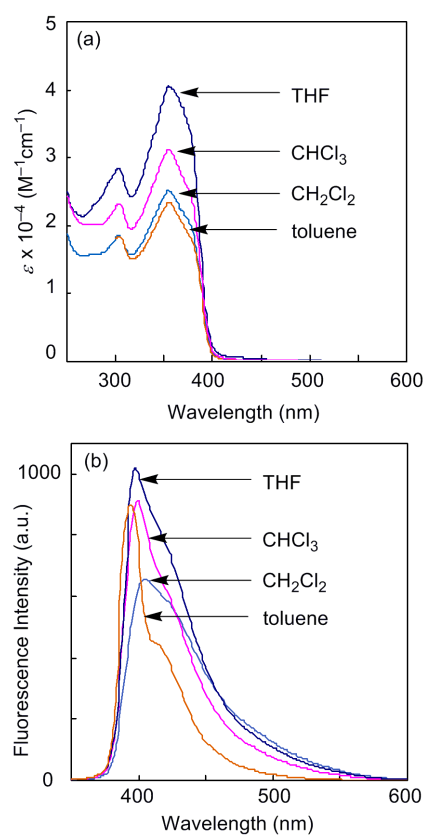
Figure 6. (a) UV-vis spectra ( c = 2.74 \times 10^{-5} \text{ M} ) and (b) fluorescence spectra ( c = 4.56 \times 10^{-7} \text{ M} ) of P1 measured in various solvents.
