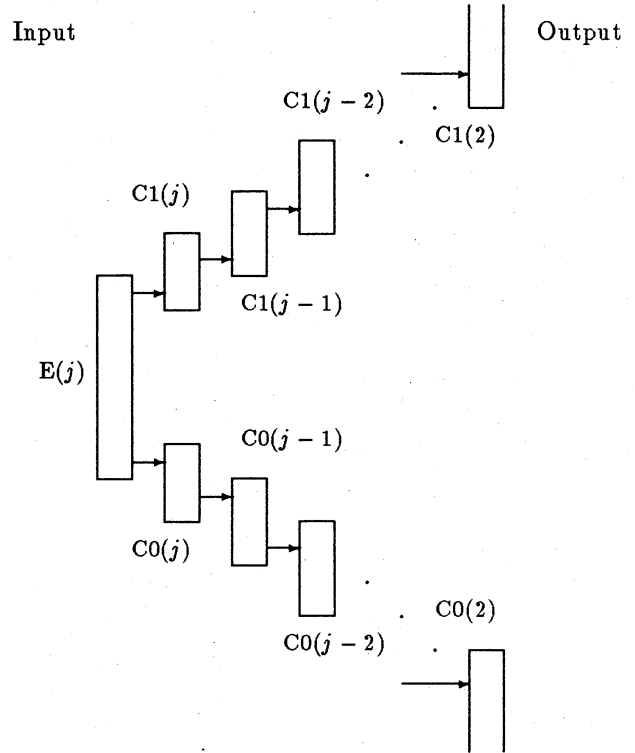
Figure 4: The structure of the layer L(j)
