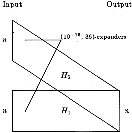
Figure 2: Construction of a (10^{-10}, 18) -expander
