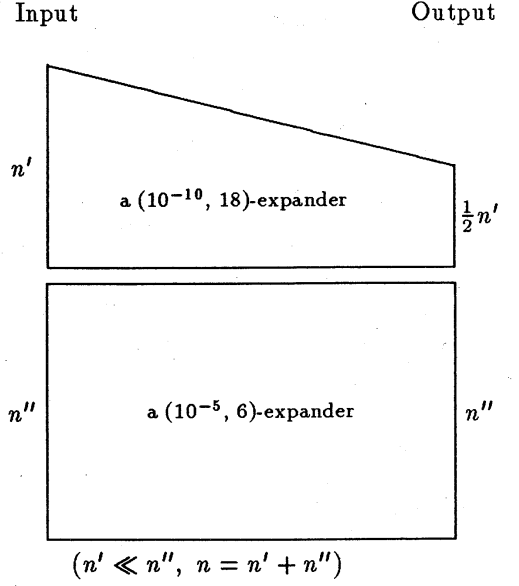
Figure 3: Construction of an (\alpha_0, 6) -expander
