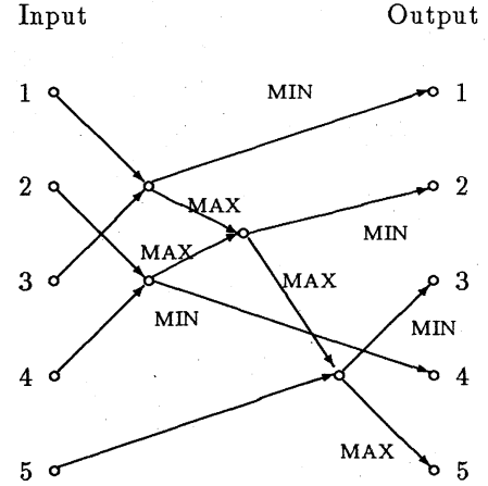
Figure 1: An example of a comparator network
