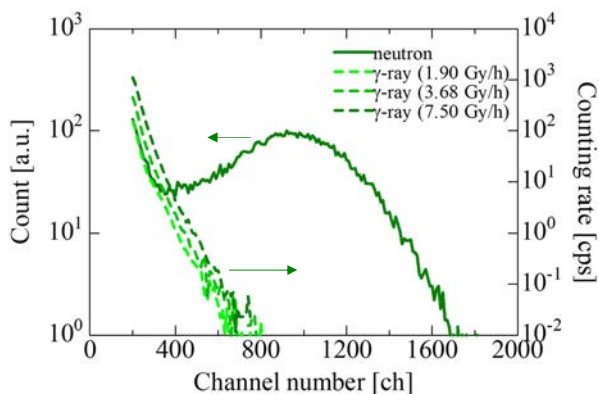
Fig. 2 Signal pulse height spectra obtained when the optical fiber type neutron detector using a Li glass scintillator of 18\ \mu\text{g} was irradiated with thermal neutrons and Co-60 gamma-rays.
