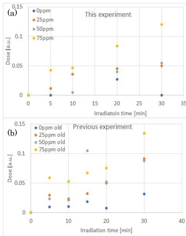
Fig. 1. Dose response dependence in the gel-dosimeter. (a): This experiment, (b): our previous study
