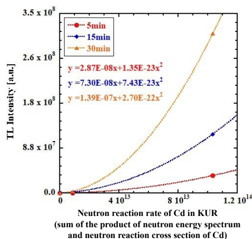
Fig.1 relationship between the neutron reaction rate of Cd in KUR and the TL amount of \text{Al}_2\text{O}_3 : Cr.
