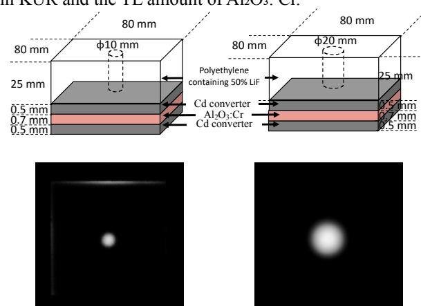
Fig.2 Upper: Arrangement of TL slabs ( \text{Al}_2\text{O}_3 : Cr using Cd converter) irradiation arrangement for TL imaging. Lower: TL image of the slab.
