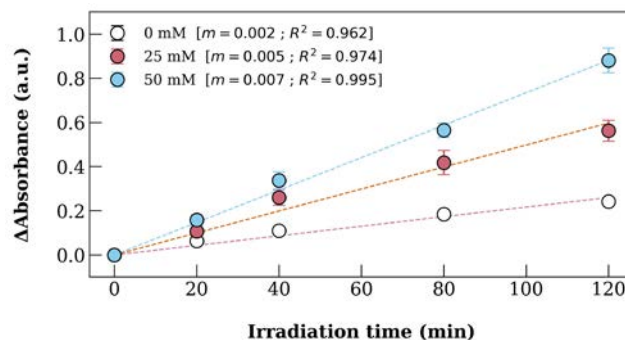
Fig. 1 Dose-response curves of PVA-GTA-I gel samples with various boric acid concentrations. All samples were measured 55 days after irradiation.
