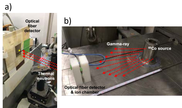
Fig. 1 Experimental setup. a) E3 port in KUR for thermal neutron irradiation. b) Co-60 gamma-ray irradiation facility in Nagoya University.
