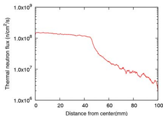
Fig. 2. Normalized thermal neutron distribution.
