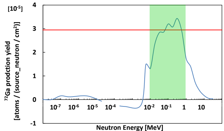
Fig. 3. Sensitivity of fast neutron detector.
