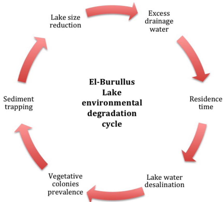
Figure 3.2: Burullus Lake environmental degradation cycle.
