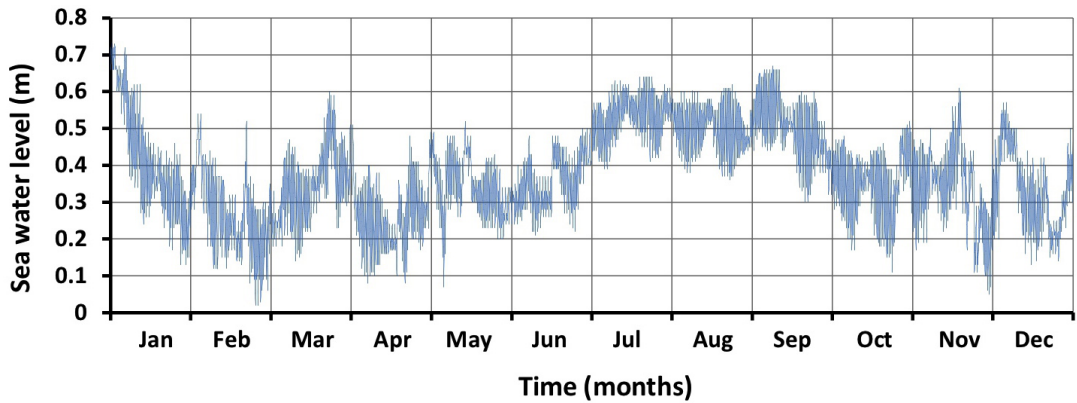
Figure 3.11: Sea water level at Burullus outlet during 2001.
