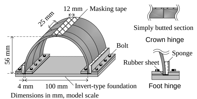
Fig. 4. Three-hinge type of arch culvert model
