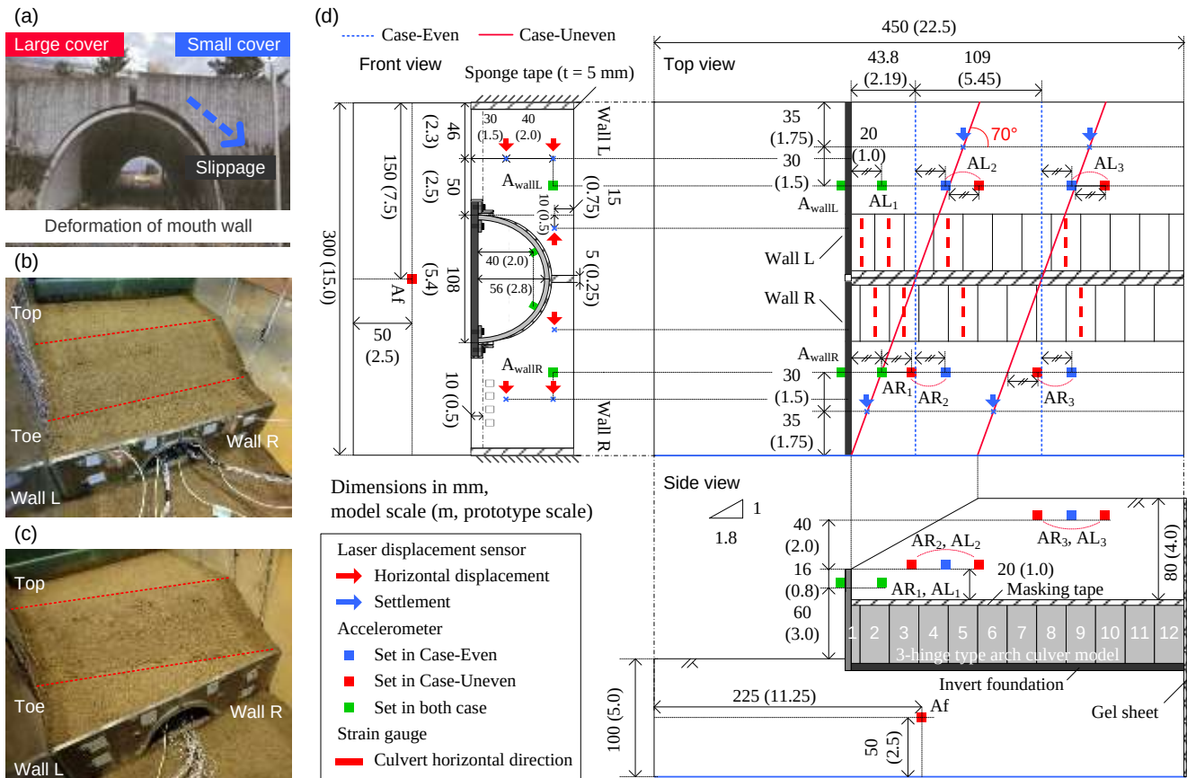
Fig. 2. Schematic drawings of experimental set-up: (a) referenced disaster example of Great East Japan earthquake (11 March 2011) cited from Abe and Nakamura (2014), (b) Case-Even, (c) Case-Uneven, and (d) experimental set-up of Case-Even and Case-Uneven.
