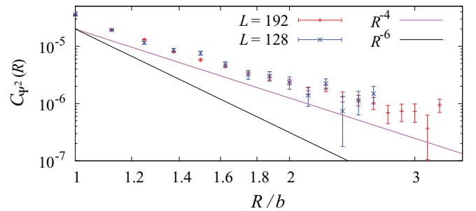
FIG. 5. (Color online) The two-point correlation function of the square of block-averaged order parameter (\bar{\Psi})^2 for the SU(3) models as a function of the distance at q = 0.3343 , which is the critical point estimated from the data of L \leq 256 . The block size b is 8.
