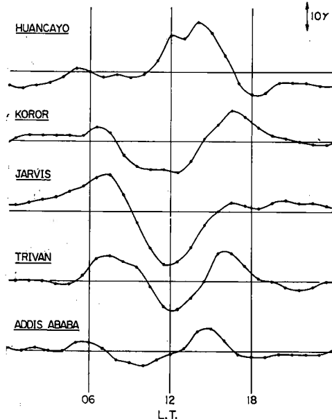
Fig. 1. The equinoctial daily variations (IGY) of D-component for five stations, Huancayo, Koror, Jarvis Island, Trivandrum and Addis Ababa.
