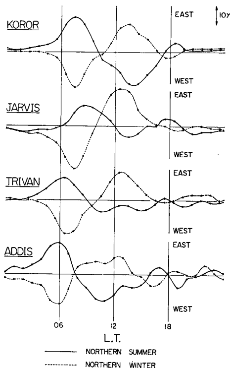
Fig. 2. The solstitial daily variations (IGY) of D-component deviated from the equinoctial daily one for four stations, Koror, Jarvis Island, Trivandrum and Addis Ababa.
