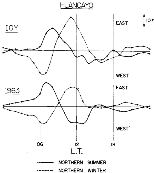
Fig. 3. The solstitial daily variations of D-component deviated from the equinoxial daily one for IGY and 1963 at Huancayo.
