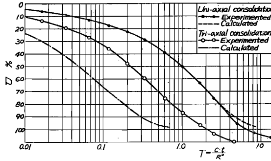
Fig. 7 Relationship between degree of consolidation and time factor (log. scale).
