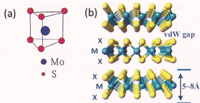
Figure 2.19 (a) Unit cell of \text{MoS}_2 , and (b) crystal structure of TMDs. (Taken from Ref. (a) [110] and (b) [19]).
