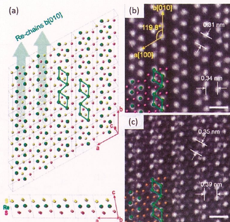
Figure 2.37 (a) Schematic of crystal structure of \text{ReX}_2 . (b) and (c) ADF images results of \text{ReX}_2 . The lattice spacing for Re diamond chains (Re diamond-shape clusters) is 0.34 nm (0.31 nm) and 0.39 nm (0.35 nm), for \text{ReS}_2 and \text{ReSe}_2 , respectively. Scale bar is 0.6 nm. (Taken from Ref. [154]).
