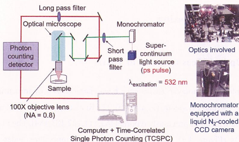
Figure 4.3 The setup of the time-resolved photoluminescence (TRPL) with TCSPC technique.
