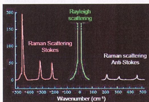
Figure 2.15 Example spectrum of Raman scattering. (Taken from Ref. [105]).
