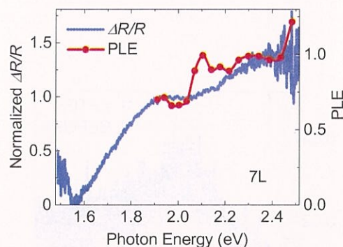
Figure 5.12 Differential reflectance ( \Delta R/R ) (blue line) and PL excitation (PLE) (red circle and line) spectra of 7L ReS 2 on the quartz substrate using the polarized excitation incident light at room temperature. The PLE spectrum is matched to the differential reflectance spectrum.
