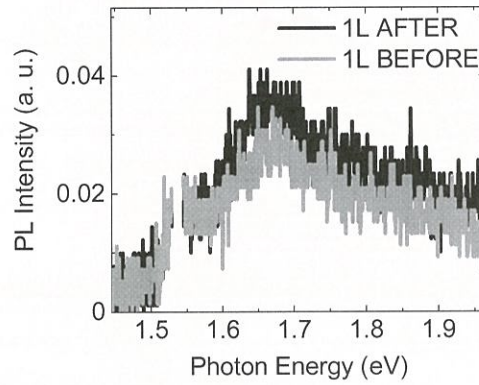
Figure 5.14 PL spectra of monolayer (1L) of \text{ReS}_2 before and after \text{F}_4\text{-TCNQ} treatment.
