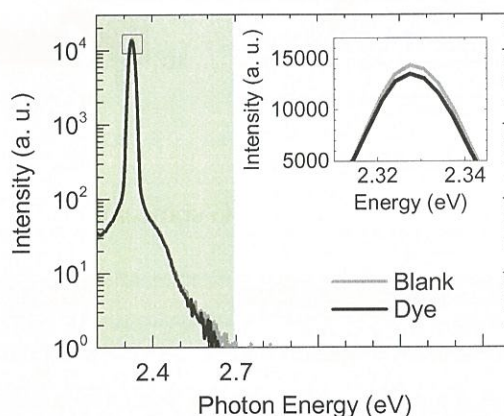
Figure 3.14 Excitation light profile of absolute QY in expended scale (inset).
