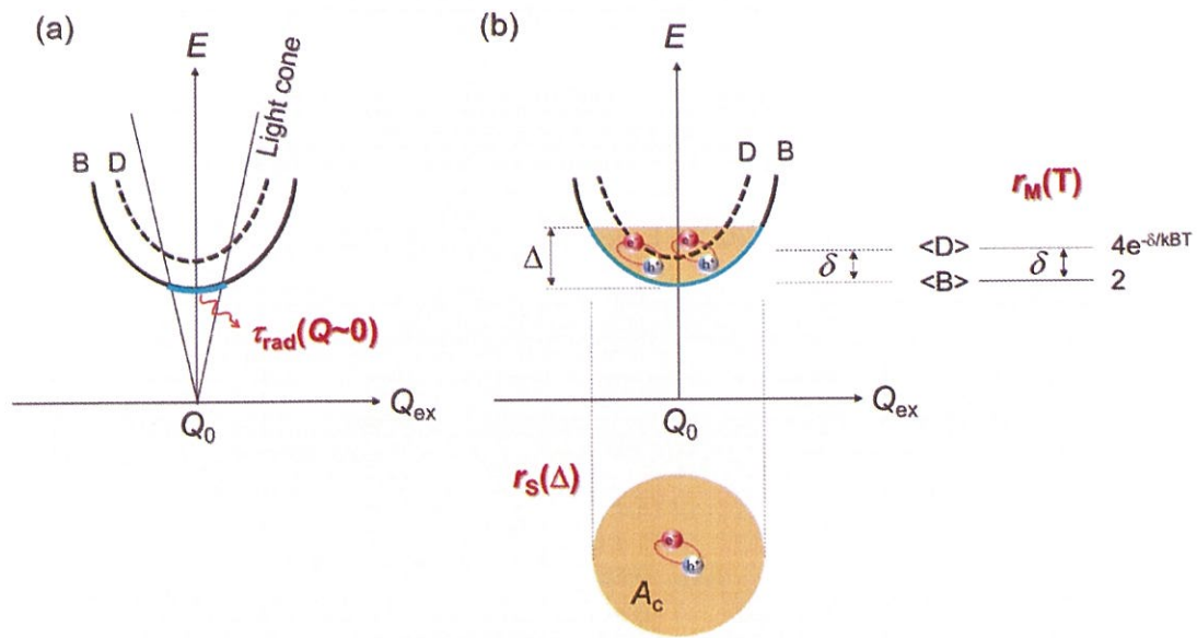
Figure 4.12 Schematic model of TMDs long effective exciton radiative lifetimes; (a) at low temperature limit, \tau_{rad}(Q \sim 0) , and (b) as a consequence of finite coherence area, A_c and population of dark exciton state, r_M , where E is energy, Q_{ex} denotes as exciton momentum, \Delta is set as the homogeneous linewidth, and the \delta is energy splitting distance between the bright (B) and dark exciton state (D).
