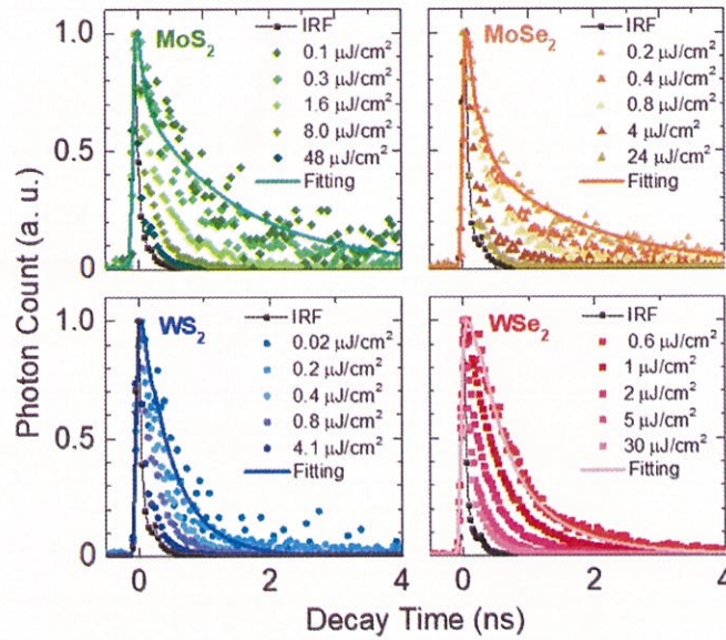
Figure 4.11 Normalized PL decay profiles of monolayer TMDs at various excitation power densities, and IRF. The solid lines correspond to the curves fitted by double-exponential functions.
