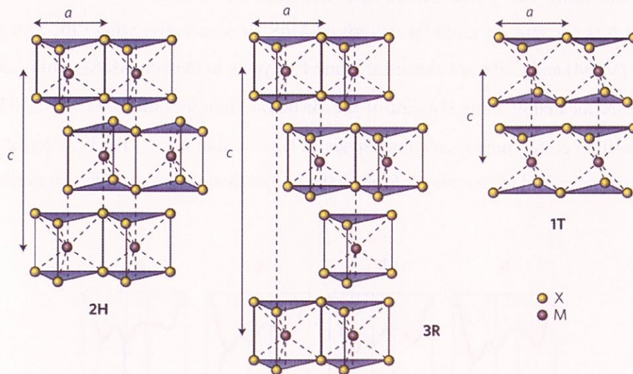
Figure 2.20 TMDs structure of polytypes, 2H (hexagonal symmetry), 3R (rhombohedral symmetry) and 1T (tetragonal symmetry). (Taken from Ref. [111]).
