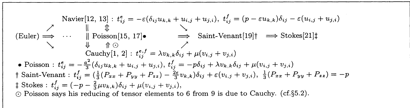
(fig.1) A genealogy of stress tensors in the prototypical Navier-Stokes equations
